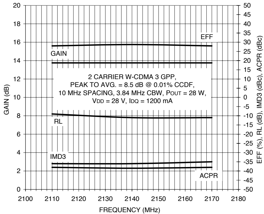
Figure 8. Broadband Performance
