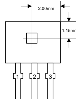
Sensor Location
