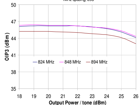
OIP3 vs. Output Power
