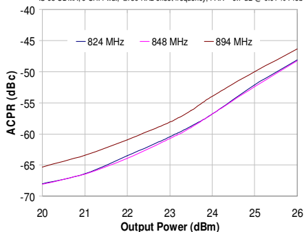
ACPR vs. Output Power
