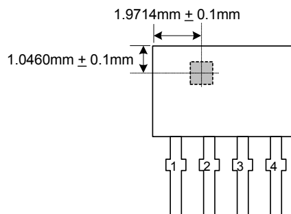
Package Dimension
