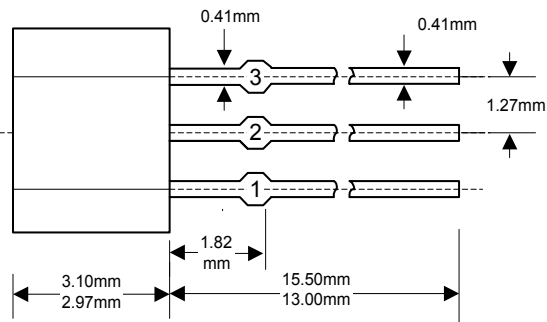
Package Dimension
