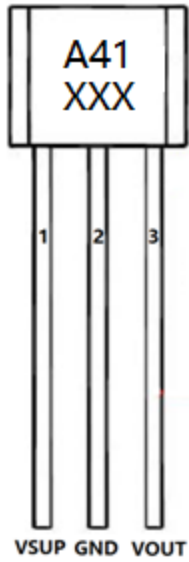
TO92S
