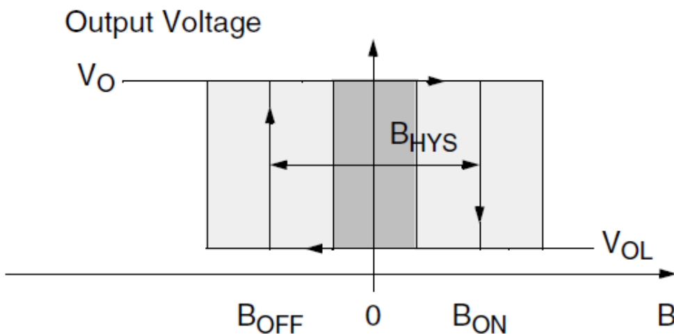
AH401UA/SU output behavior
