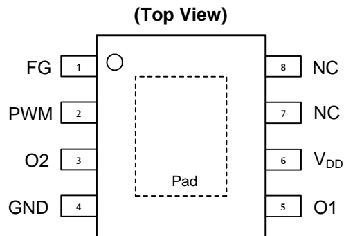
MSOP-8EP
