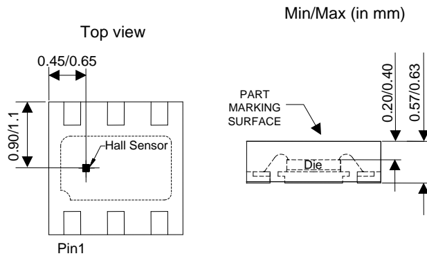
Sensor Location
