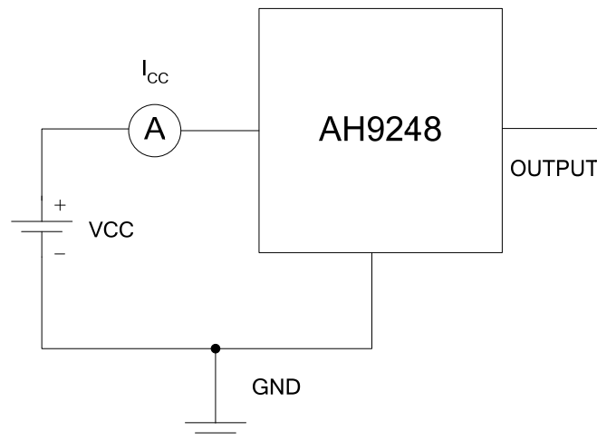
Figure 5. Average Supply Current (Note 5, 6)
