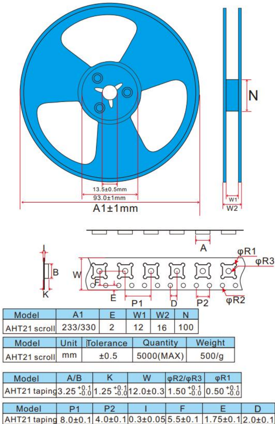
Figure 22. Package tape and sensor location diagram.
