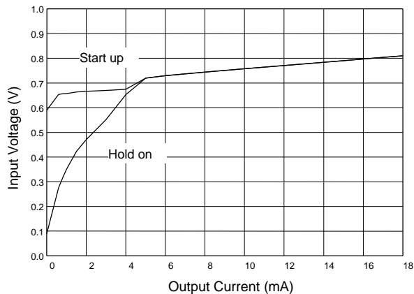
Fig. 3 AIC1642-27 Start-up & Hold-on Voltage (L=100 \mu H)
