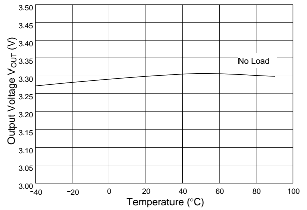
Fig. 20 AIC1642-33 Output Voltage vs. Temperature
