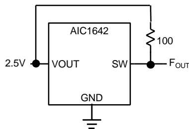
Oscillator Test Circuit
