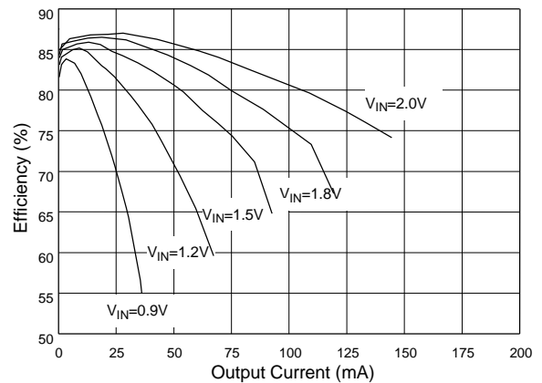
Fig. 18 AIC1642-33 Efficiency (L=100μH CD54)
