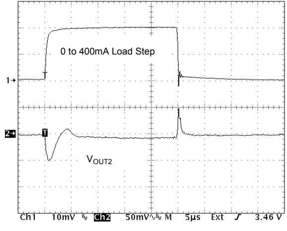
FIG. 7 Transient Response of Linear Regulator
