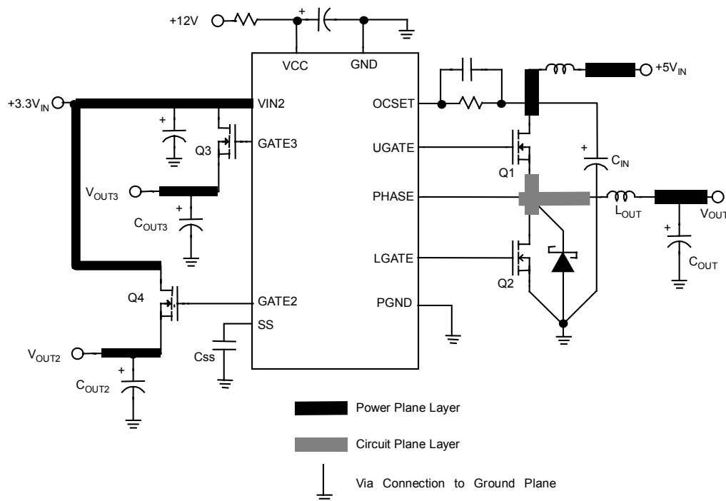
Fig. 18 Printed circuit board power planes and islands
