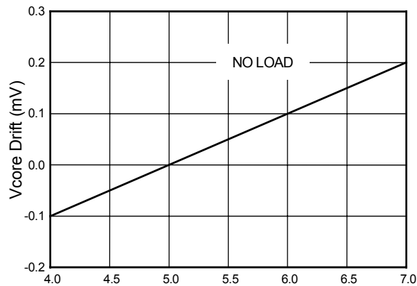
FIG.16 Vcore Drift vs. VIN (V)
