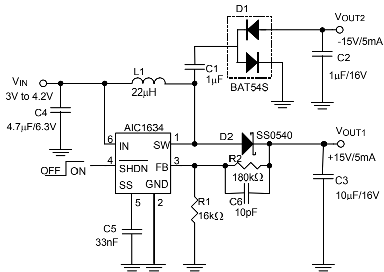
Fig. 19 1-Cell Li-Ion to \pm 15V/5mA Dual Output Converter for LCD Bias
