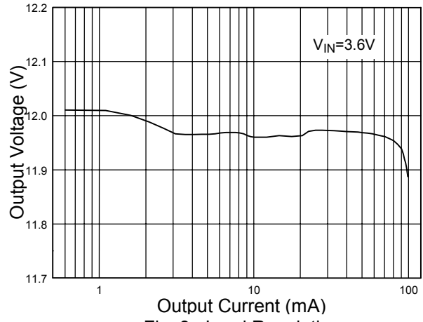
Fig. 3 Load Regulation
