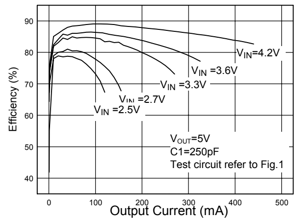
Fig. 5 Efficiency vs. Output Current
