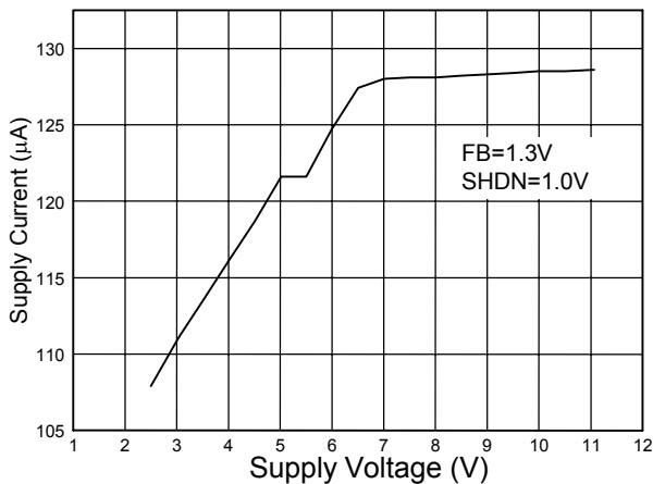
Fig. 4 Non-Switching Current
