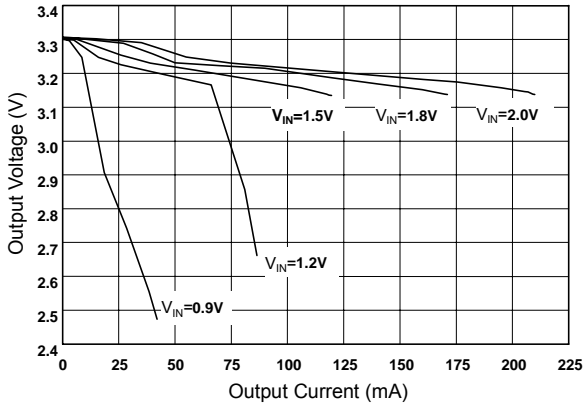
AIC1638-33 Load Regulation (L=47μH, CD54)
