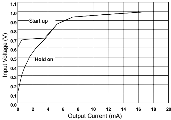
AIC1638-33 Start-up & Hold-on Voltage (L=100μH)
