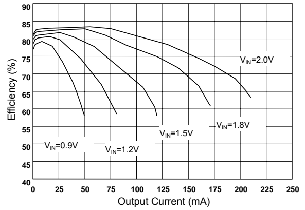
AIC1638-33 Efficiency (L=47μH, CD54)
