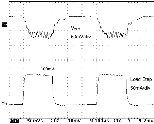
Load Transient Response (L=100µH, Co=47µF, VIN=2V)
