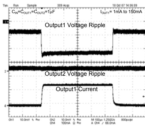
Fig. 21 Cross talk at V_{IN}=3.8V , V_{OUT1}=1.8V , V_{OUT2}=2.8V , I_{OUT2}=150mA
