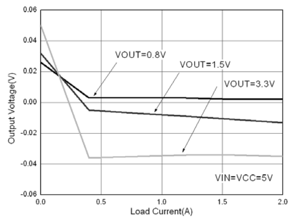
Fig. 10 Output Voltage Deviation vs Load Current
