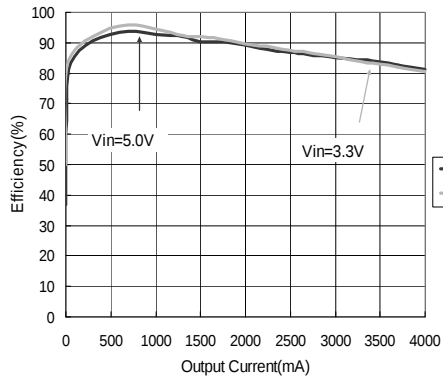
Fig. 1 Efficiency(%) V.S. Load Current(mA) ( V_{CC} = V_{IN} , V_{OUT} = 1.8\text{V} )
