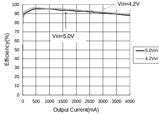
Fig. 2 Efficiency(%) V.S. Load Current(mA) ( V_{CC} = V_{IN} , V_{OUT} = 3.3\text{V} )
