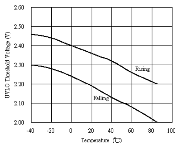
Fig. 10 UVLO Threshold Voltage vs. Temperature
