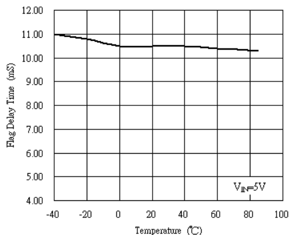
Fig. 8 Flag Delay Time vs. Temperature
