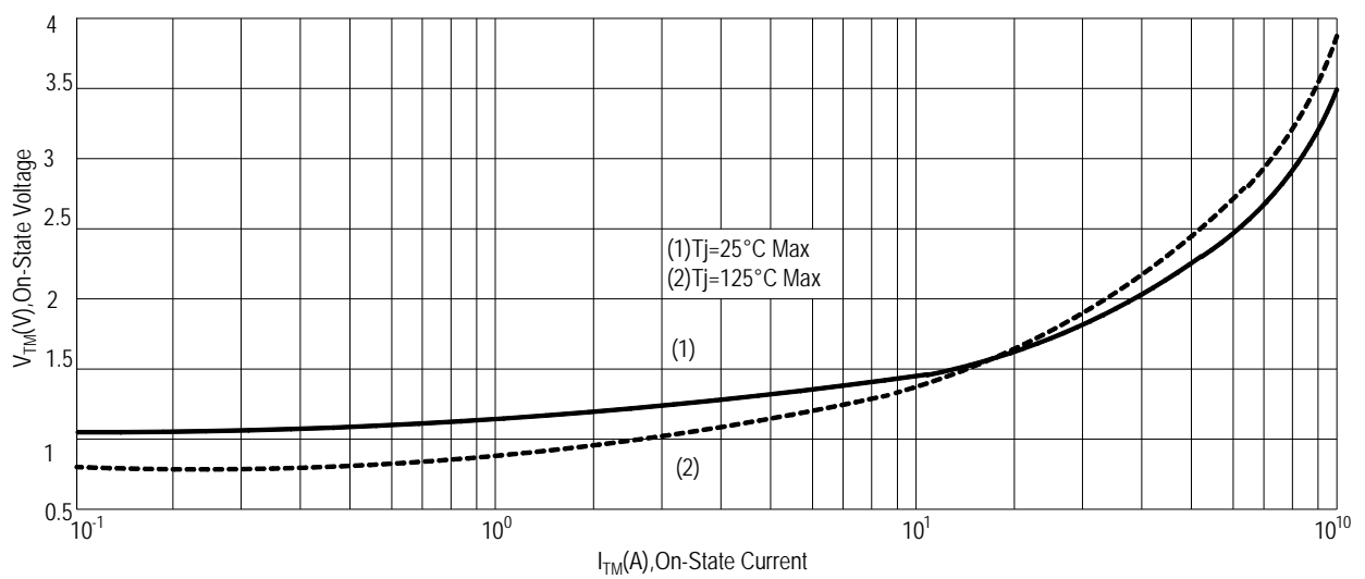
FIG.9: On-state characteristics(Max)
