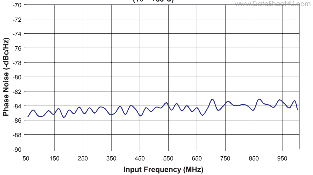
Figure 10: Composite Oscillator Phase Noise @ 10 KHz Offset (T c = +55°C)
