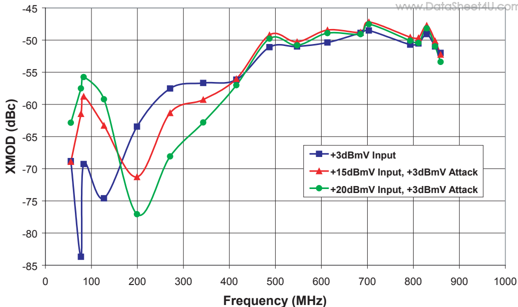
Figure 8: XMOD vs. Frequency (129 channels - flat, T c = +55°C)
