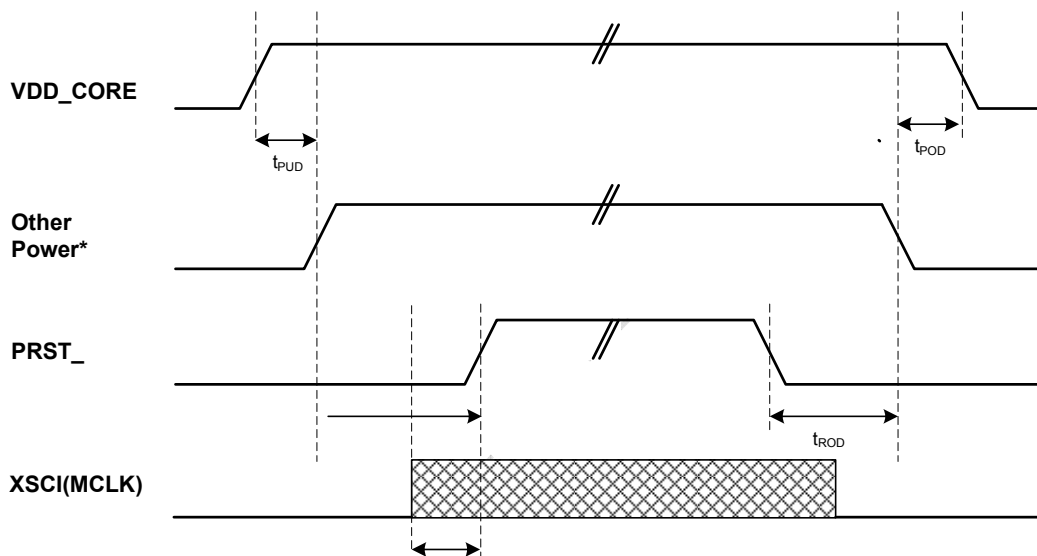
Figure 5. Power on/off timing diagram
