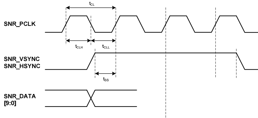
Figure 3. Parallel sensor interface timing
