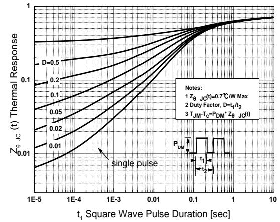
Transient Thermal Response Curve For AJCS10N65CT
