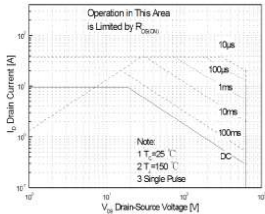
Maximum Safe Operating Area For AJCS10N65CT
