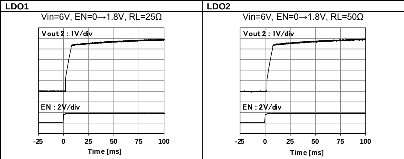
Figure 246. Starting Characteristic
