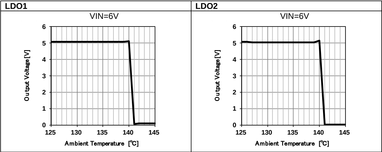
Figure19. Thermal Protection
