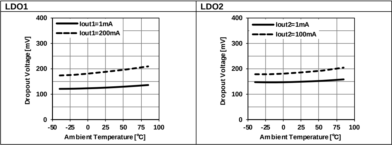
Figure 202. Dropout Voltage
