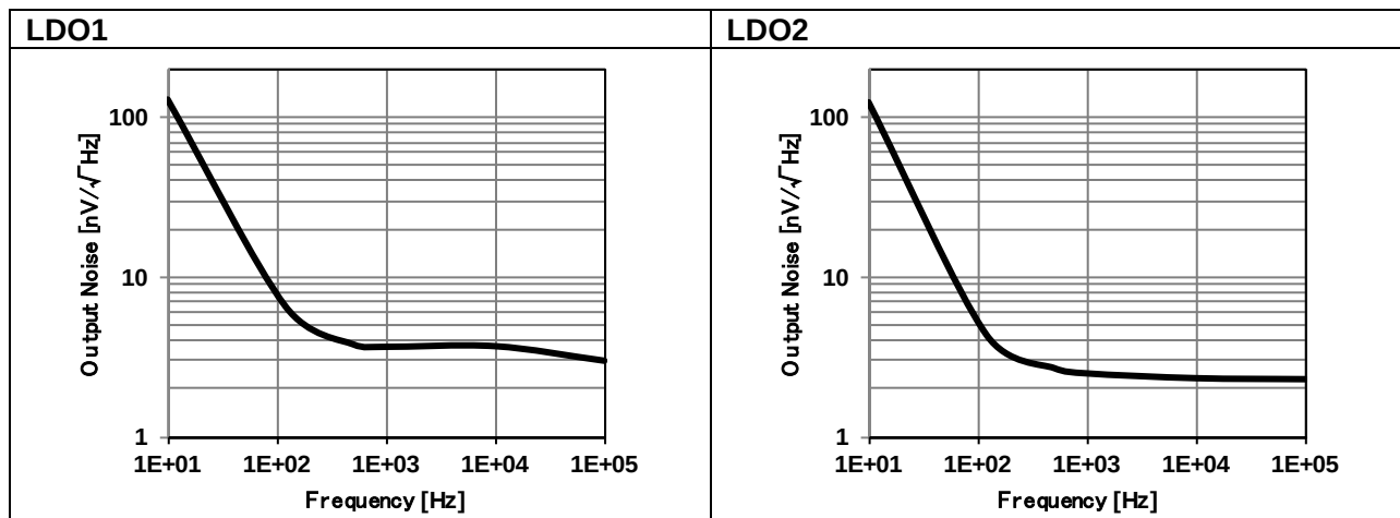
Figure 8. Output Noise Level (1/f)
