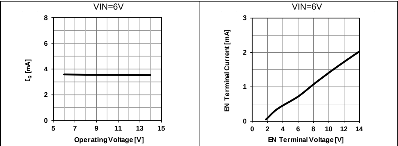
Figure 156. Quiescent Current
