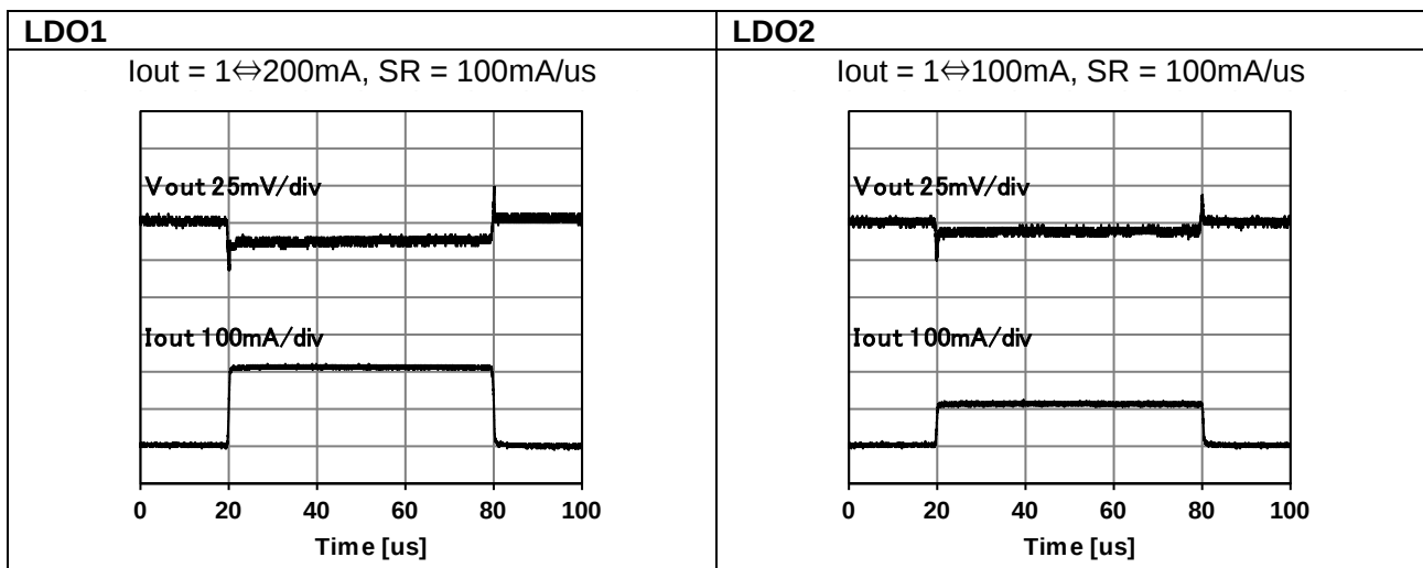
Figure 268. Load Transient
