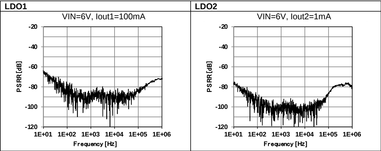
Figure 98. Ripple Rejection
