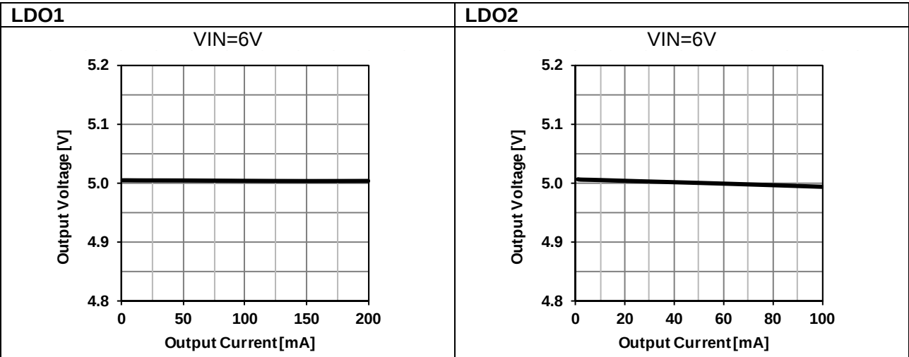
Figure 112. Load fluctuation
