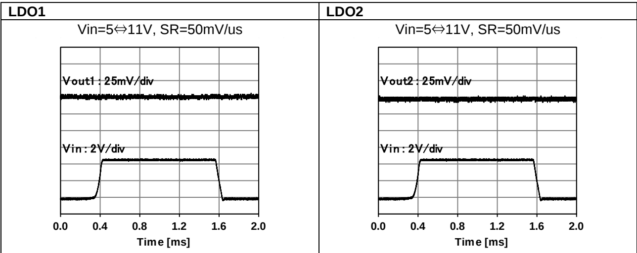
Figure 25. Line Transient
