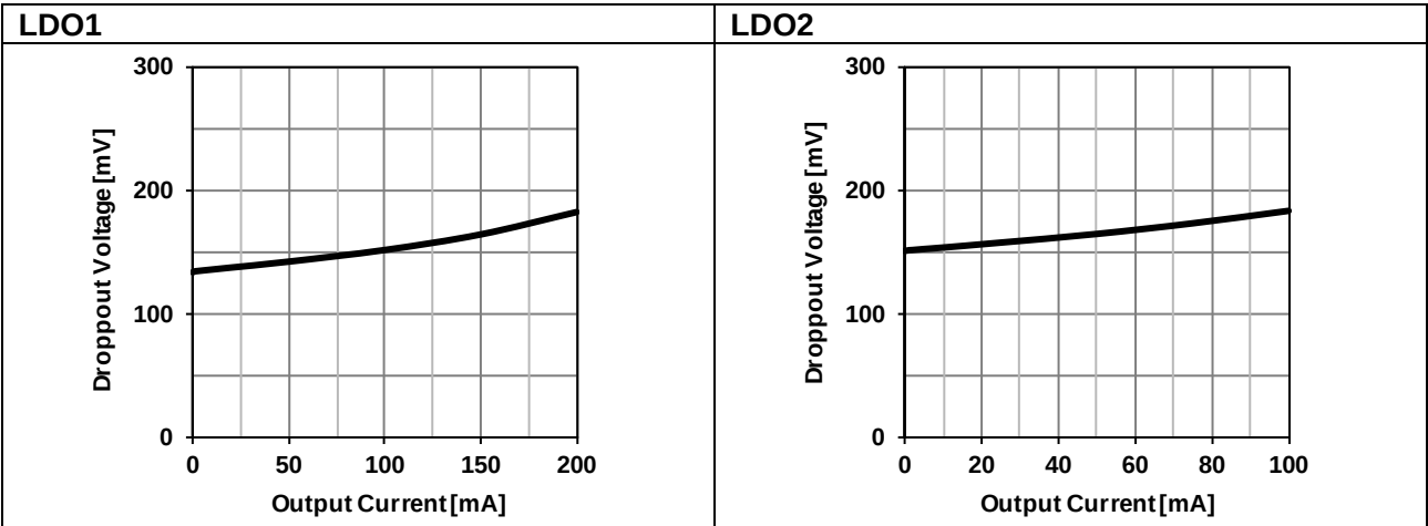
Figure 134. Dropout Voltage
