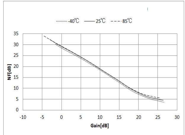
Fig.5-2 NF VS Gain (fo=165MHz)
