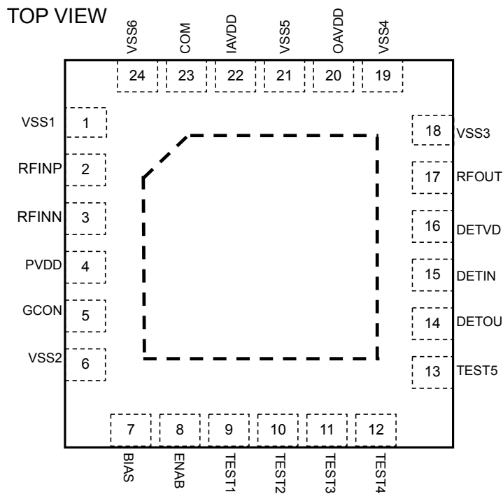
Fig 2 Pin Configuration
