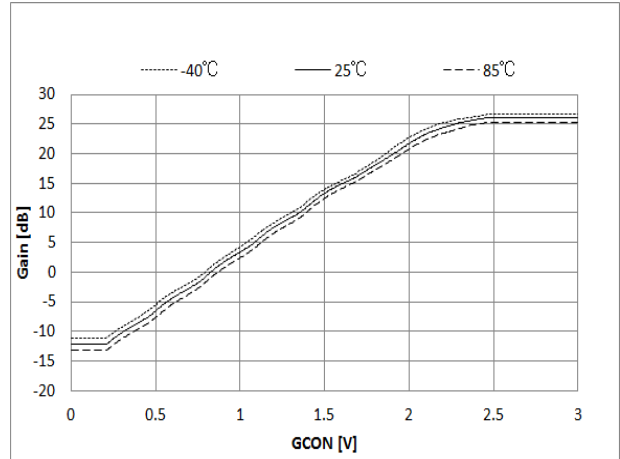
Fig.4-1 Gain VS Control Voltage(fo=165MHz)
