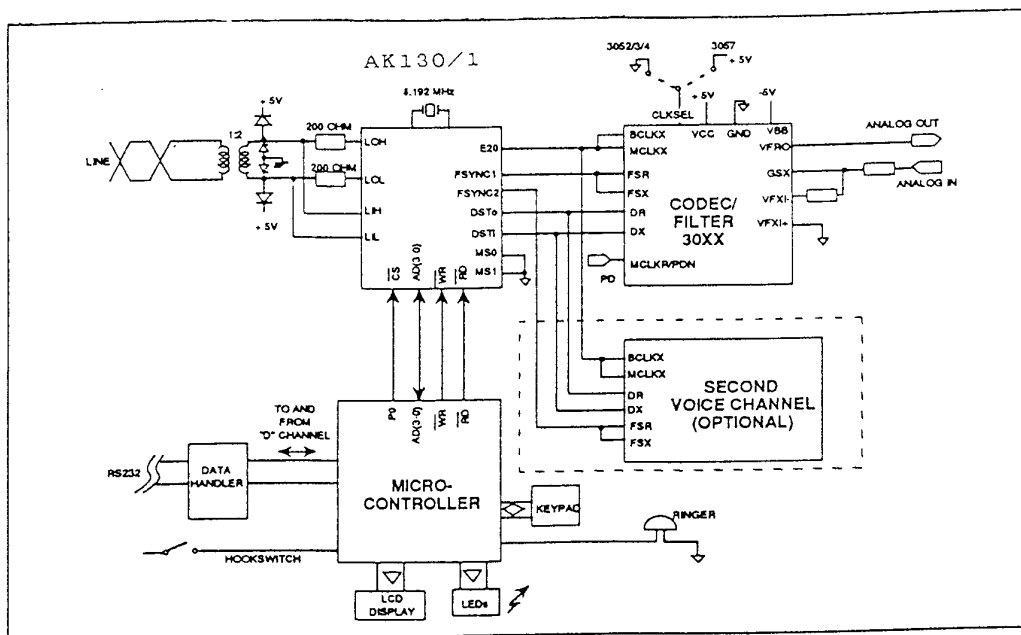
Fig-10 Typical Application - Single or Dual Voice Terminal
