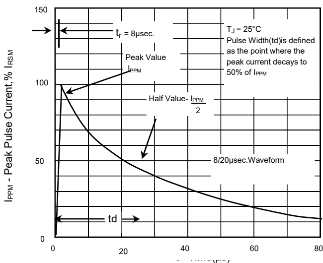
Fig.1 - Test Pulse Waveform
