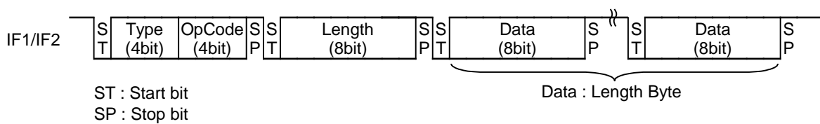
Figure.10 UART command/event format
