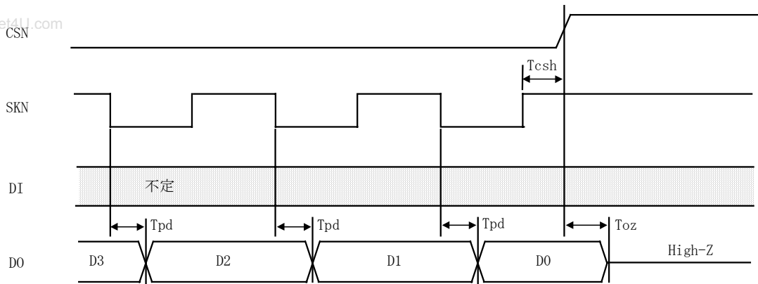
Figure 4: data output timing
