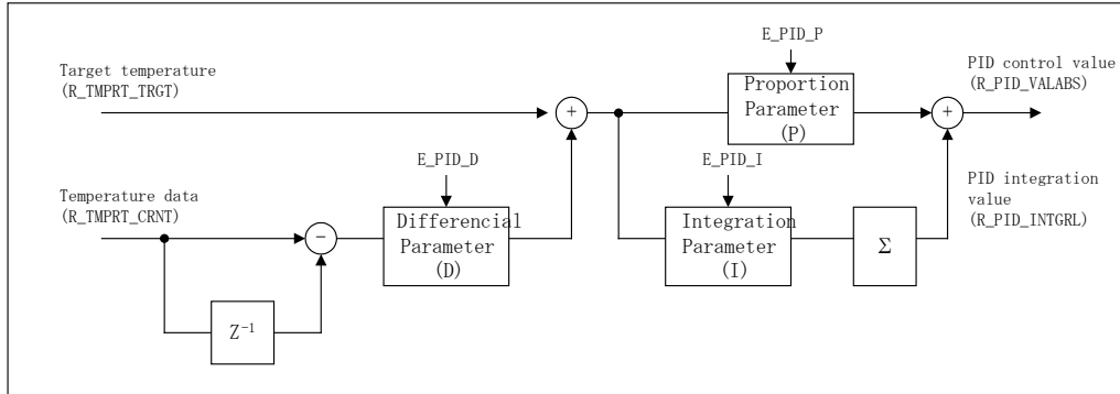
Figure 4-2 PID control
