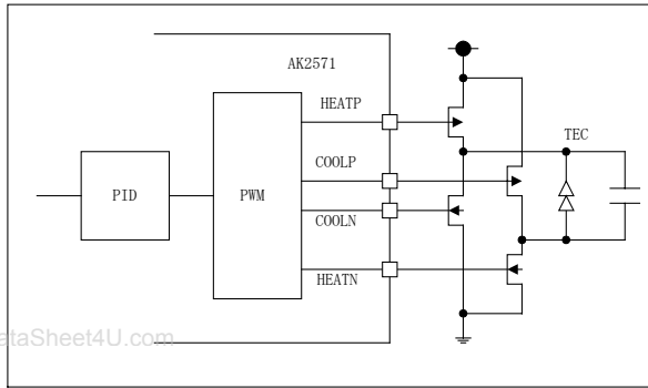
Figure 4-4 Analog control-1
