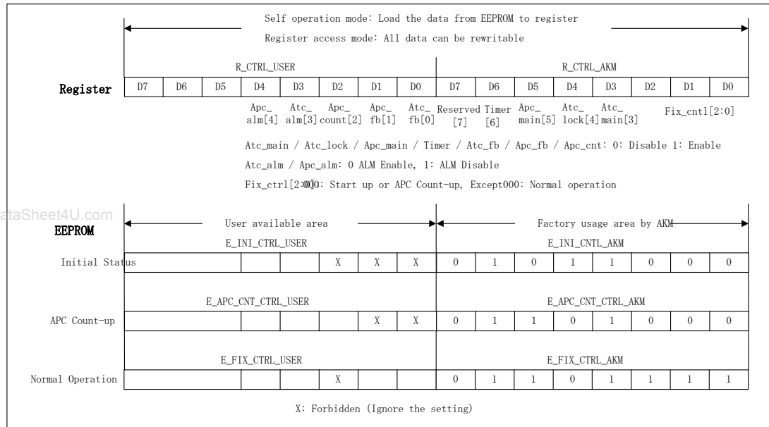
Figure 5-3 Control Register
