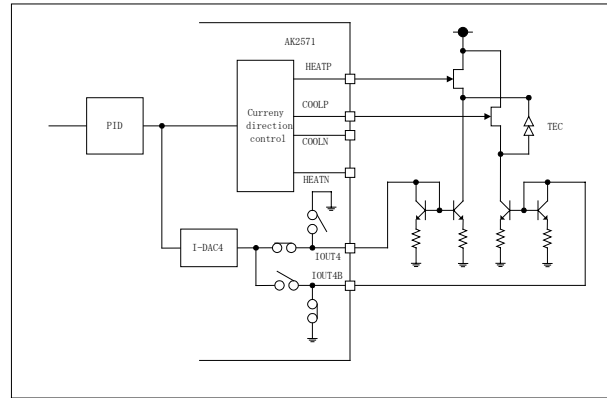
Figure 4-6 Analog control 2-2
