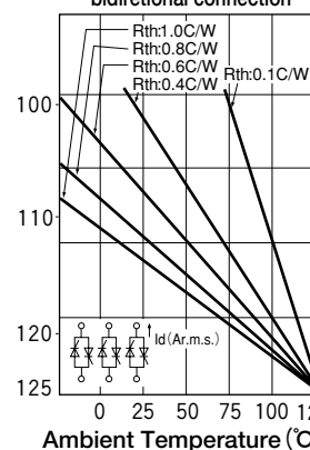
W3; Three phase bidirectional connection
