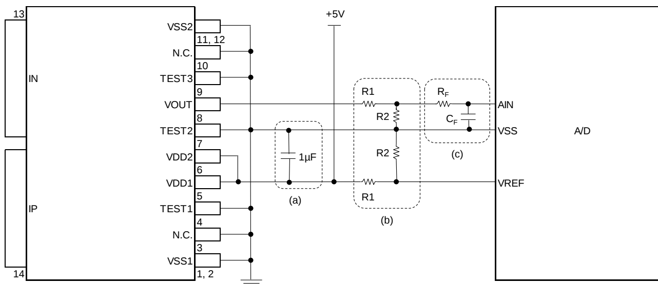
Figure 6. Recommended external circuits of AK3102
