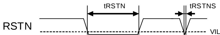
Figure 2. Reset Timing Diagram
