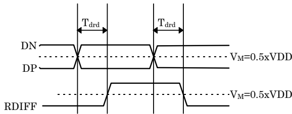
Figure Differential Receiver Delay
