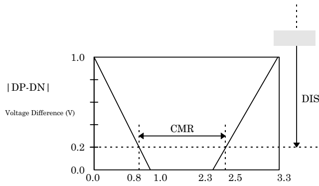
Figure Differential Input Sensitivity
