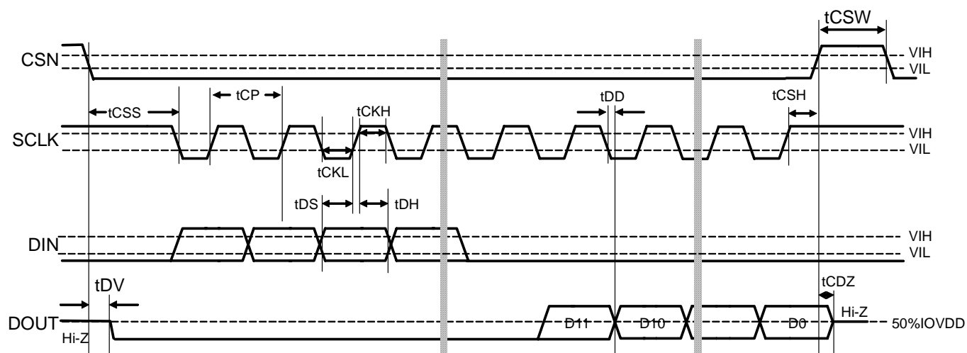
Figure 2. Timing Diagram
