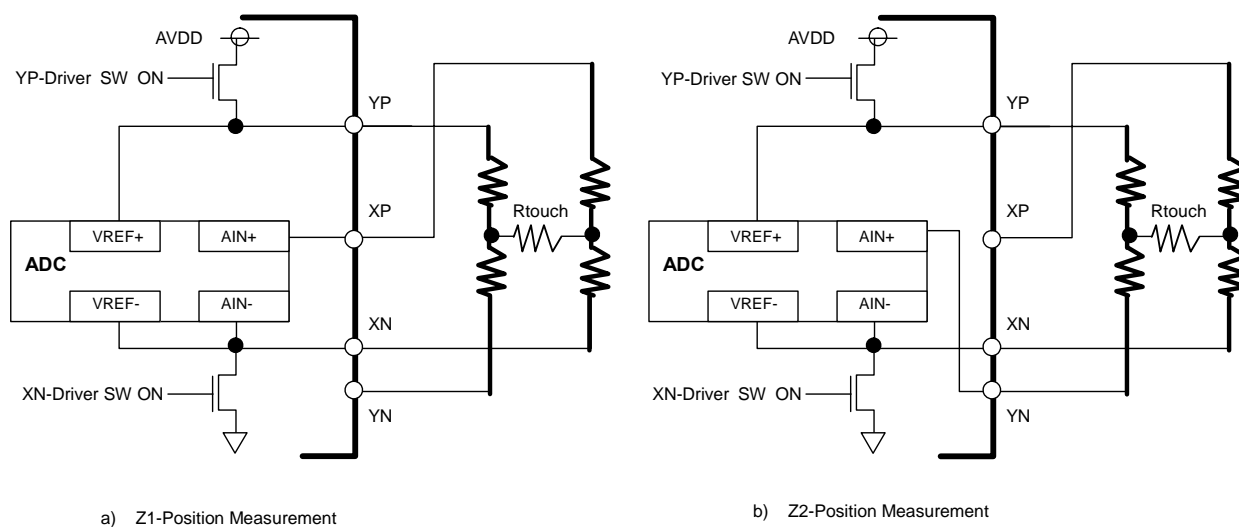
Figure 5. Pen Pressure Measurements
