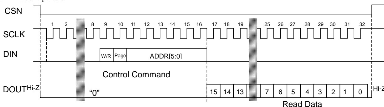
Figure 12. Read Operation
