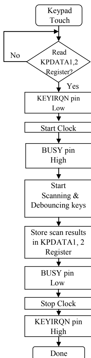
Figure 21. Keypad scanner sequence initiated by key press
