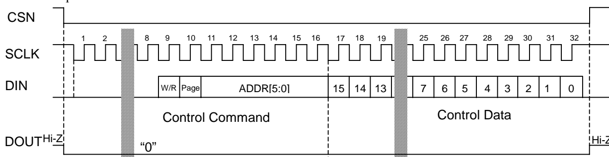
Figure 11. Write Operation
