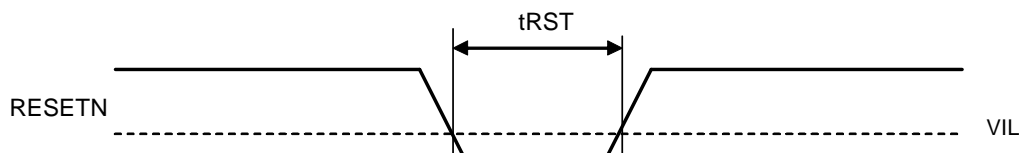
Figure 3. Power-down & Reset Timing
