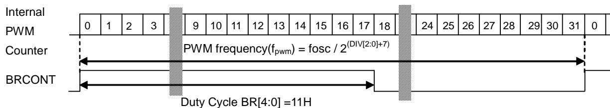
Figure 17. PWM output waveform
