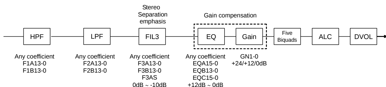
Figure 46. Digital EQ/HPF/LPF (default)
