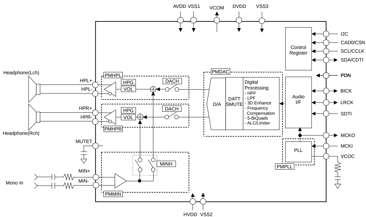
Figure 2. Block Diagram (Differential mode, HPBTL bit = "1", PSEUDO bit = "0")
