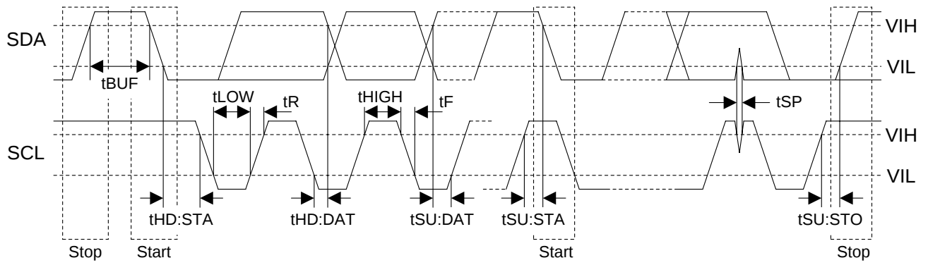
Figure 22. I²C Bus Mode Timing
