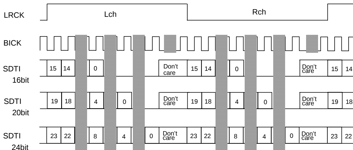
Figure 36. Mode 2 Timing
