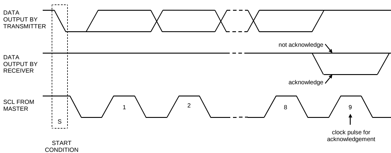
Figure 66. Acknowledge on the I 2 C-Bus
