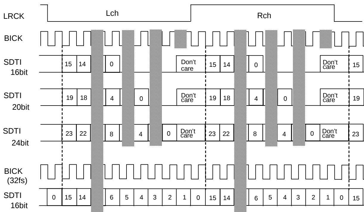
Figure 37. Mode 3 Timing
