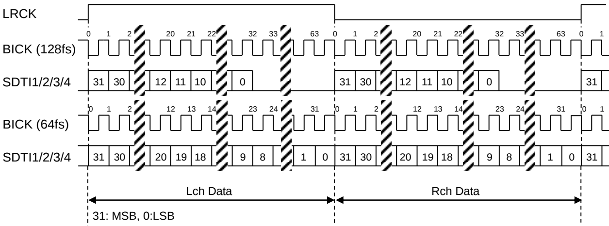
Figure 27. Mode 6 Timing
