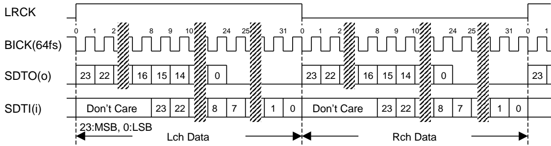
Figure 22. Mode 4/12 Timing
