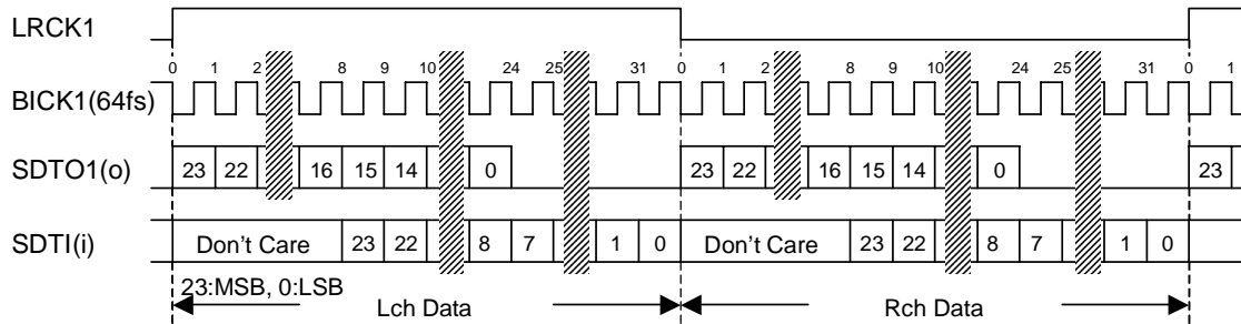
Figure 2. Mode 1,5 Timing
