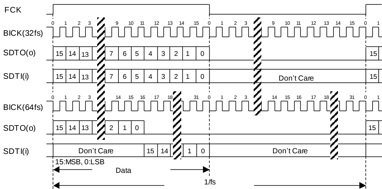
Figure 23. Mode 1 Timing
