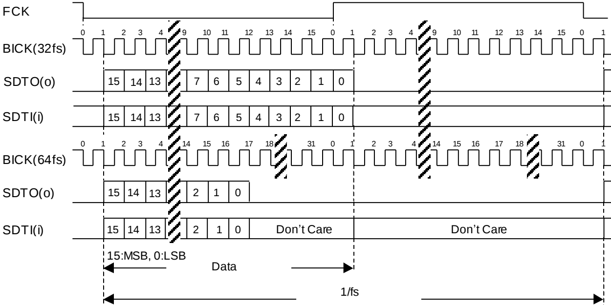
Figure 25. Mode 3 Timing
