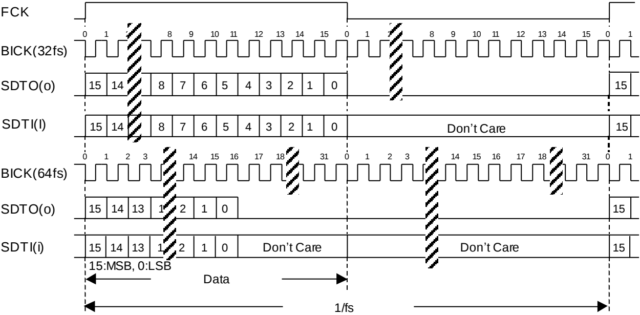
Figure 24. Mode 2 Timing
