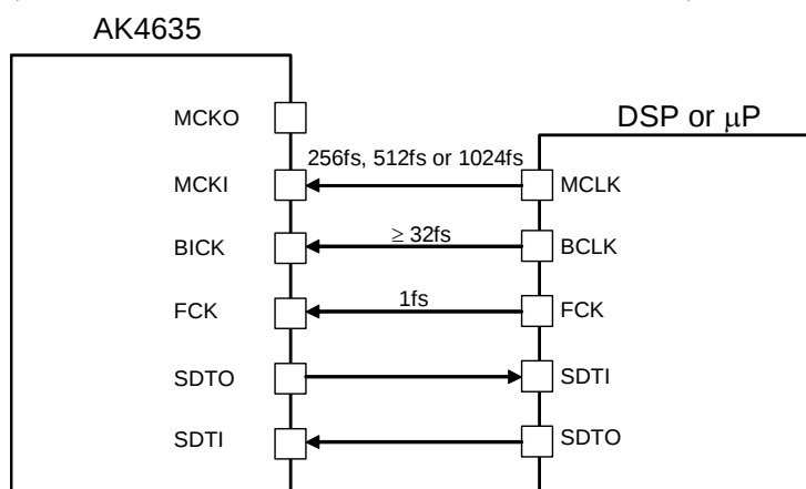
Figure 27. EXT Slave Mode
