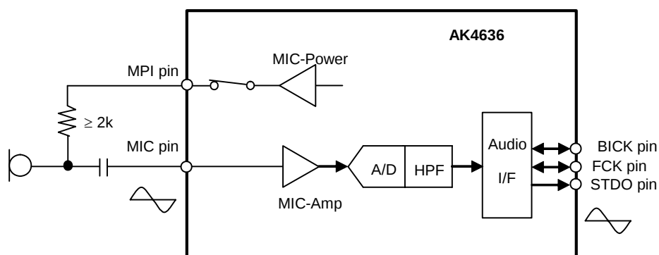
Figure 37. MIC Block Circuit
