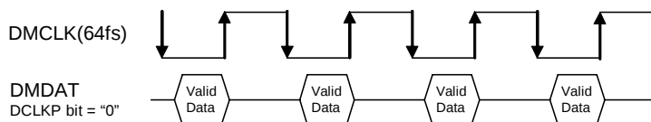
Figure 42. Data In/Output Timing with Digital MIC (DCLKP bit = “0”)
