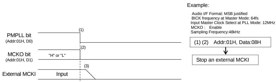
Figure 80. Clock Stopping Sequence (1)
