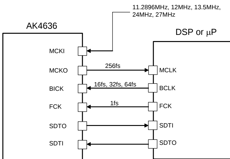
Figure 25. PLL Slave Mode 1 (PLL Reference Clock: MCKI pin)
