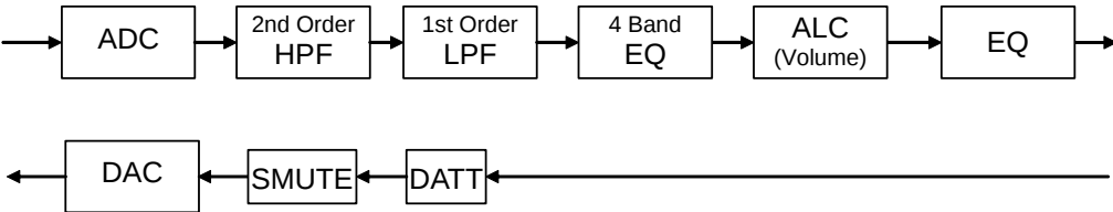
Figure 44. Path at Recording Mode (default)
