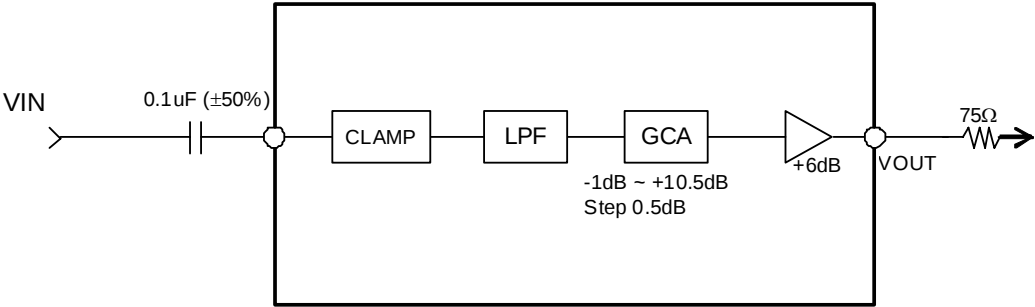
Figure 54. Video Block
