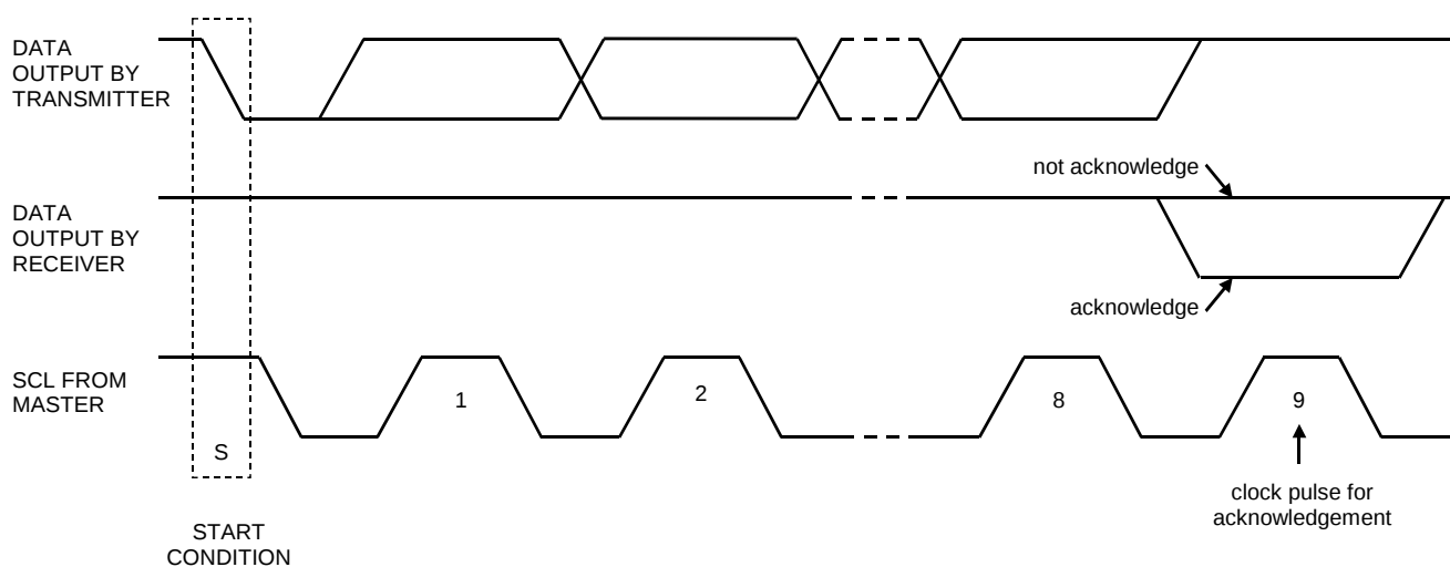
Figure 63. Acknowledge on the I 2 C-Bus
