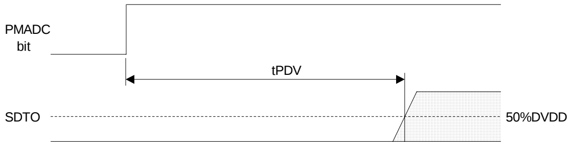
Figure 19. Power Down & Reset Timing 1
