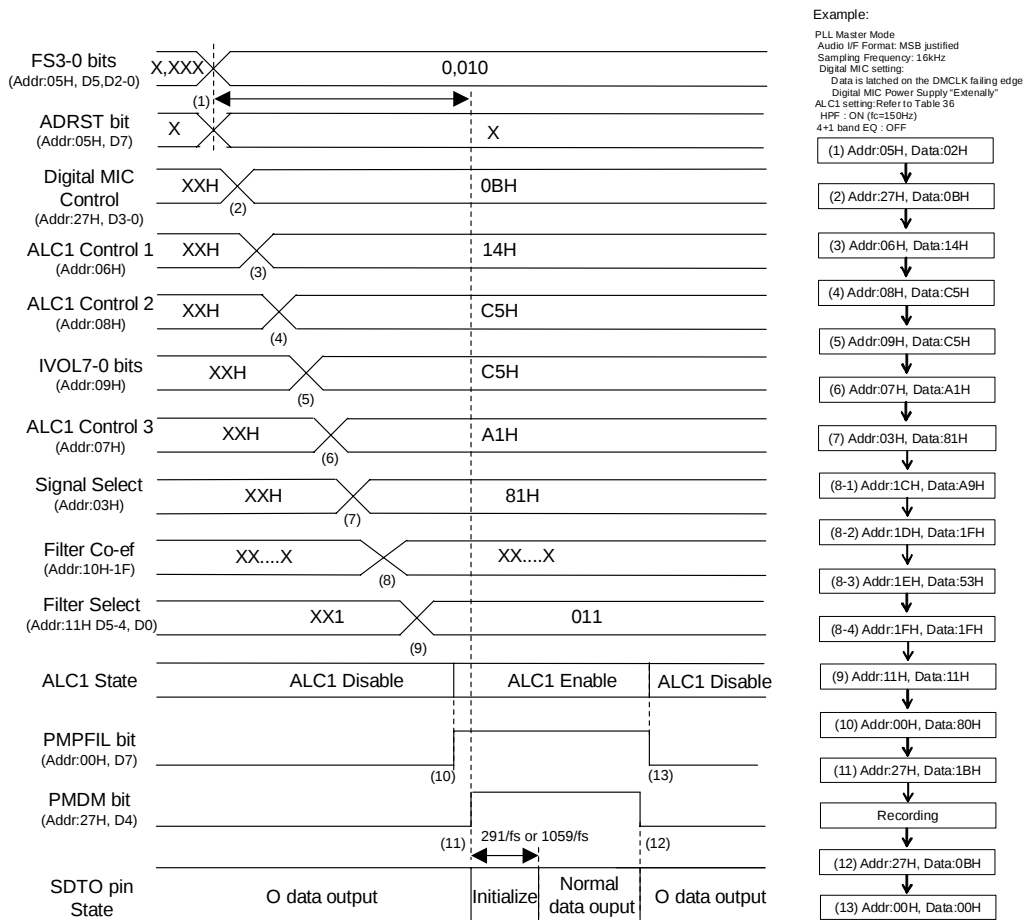
Figure 74. Digital MIC Input Recording Sequence
