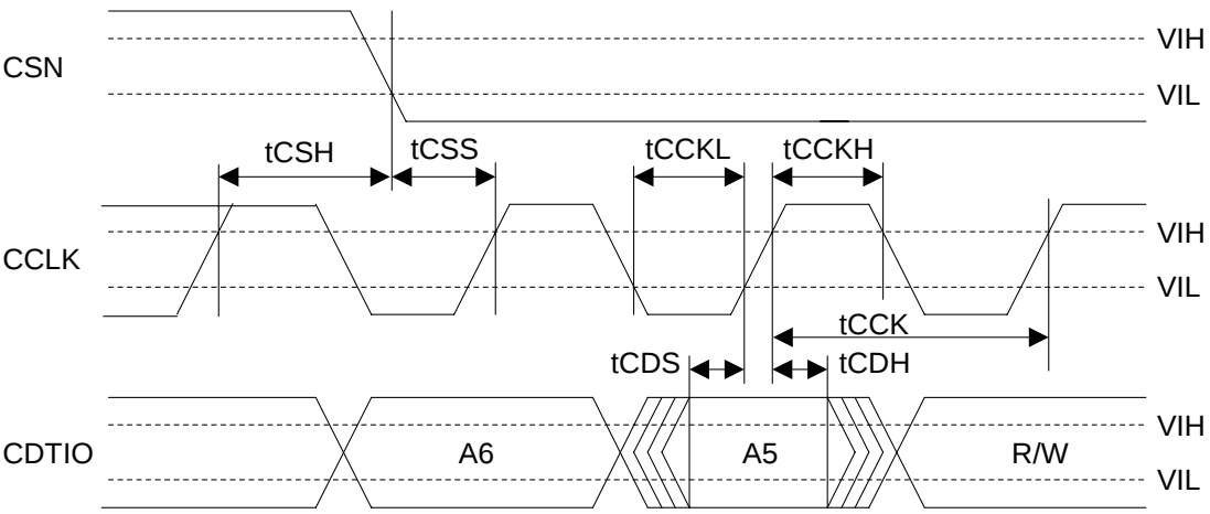
Figure 15. WRITE Command Input Timing
