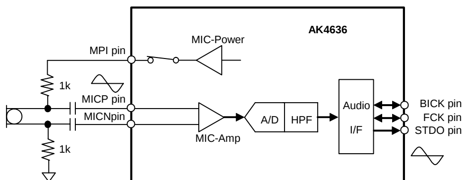
Figure 38. MIC Block Circuit (Differential; MDIF = "1")
