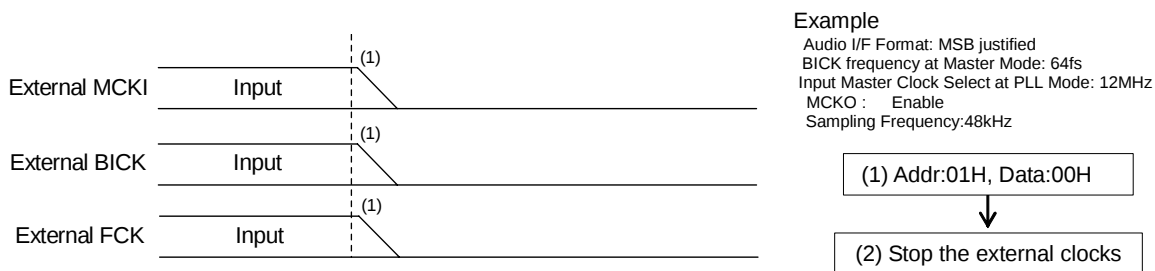
Figure 83. Clock Stopping Sequence (4)
