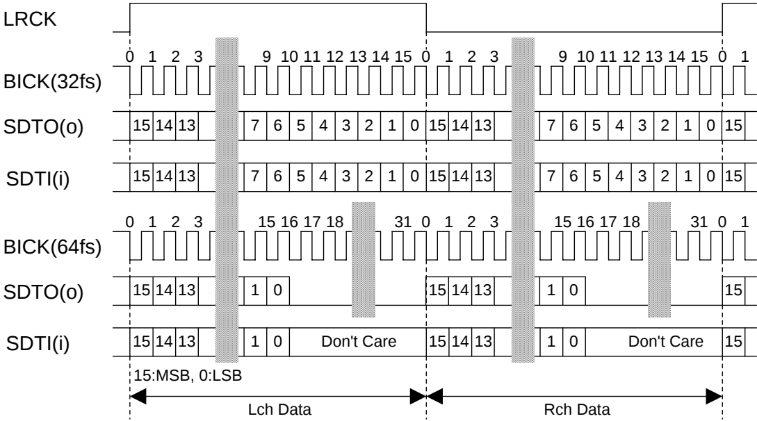
Figure 50. Mode 2 Timing
