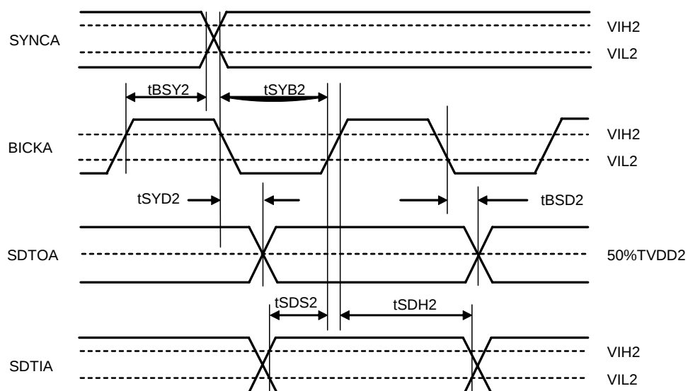
Figure 17. PCM I/F A Timing at MSB justified and I²S (Slave mode)
