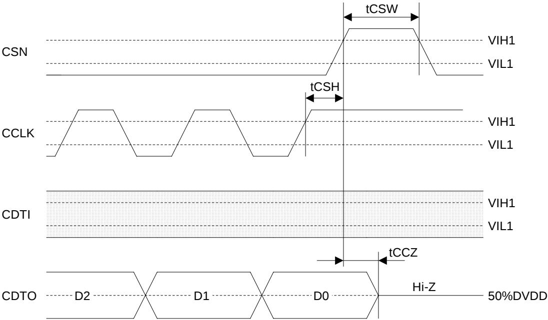
Figure 33. READ Data Output Timing 2
