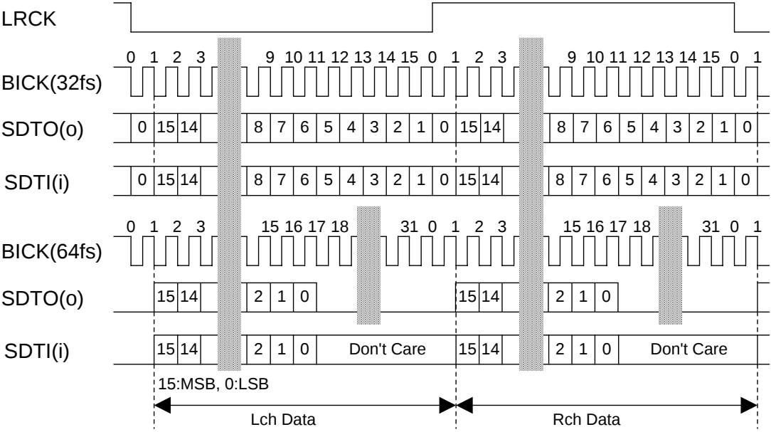
Figure 51. Mode 3 Timing
