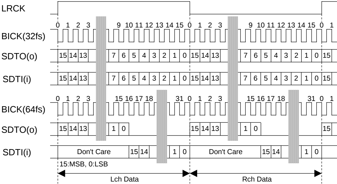
Figure 49. Mode 1 Timing
