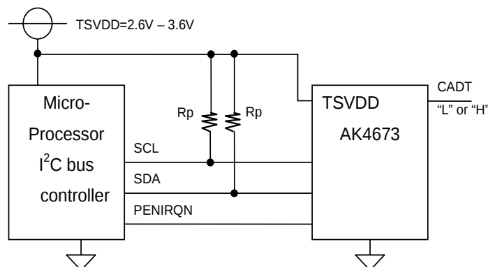
Figure 65 Digital I/F
