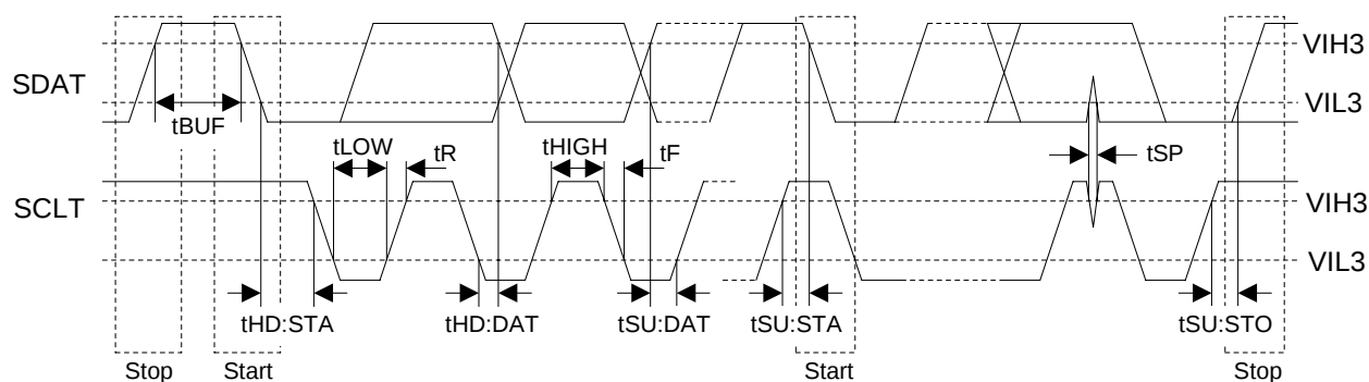
Figure 15. I²C Bus Mode Timing (TSC)
