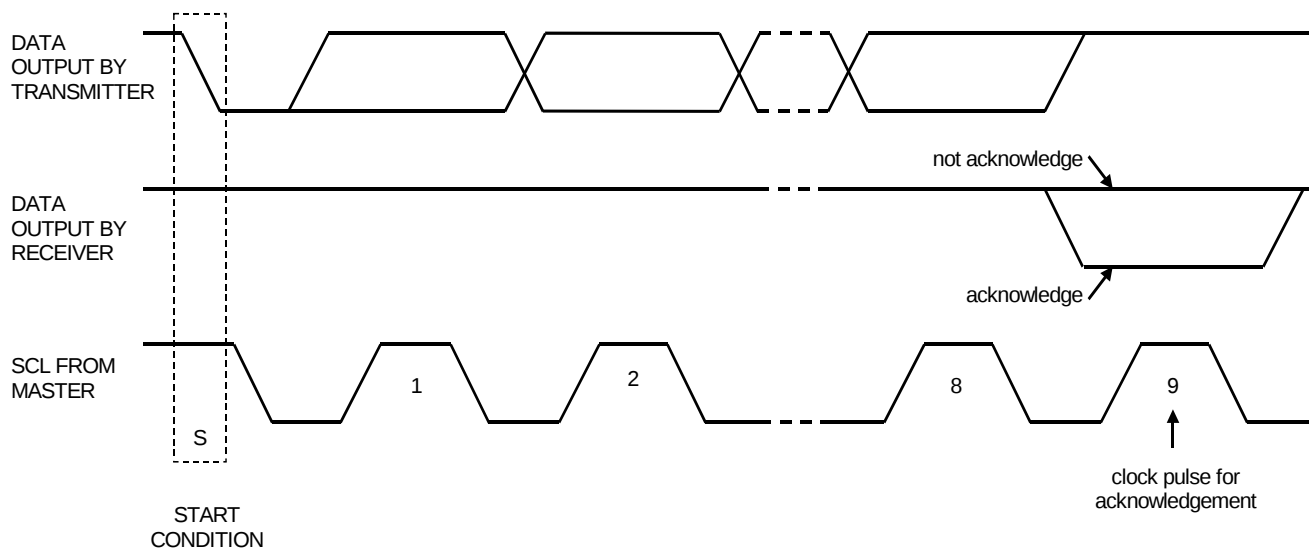
Figure 68 Acknowledge
