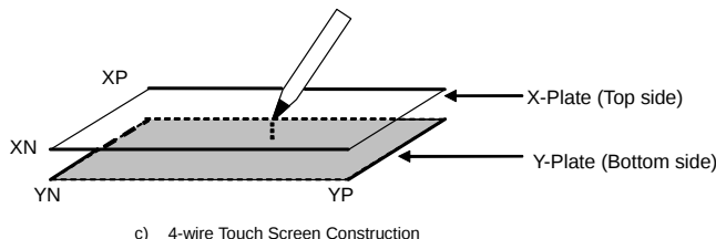
Figure 63 Axis Measurements
