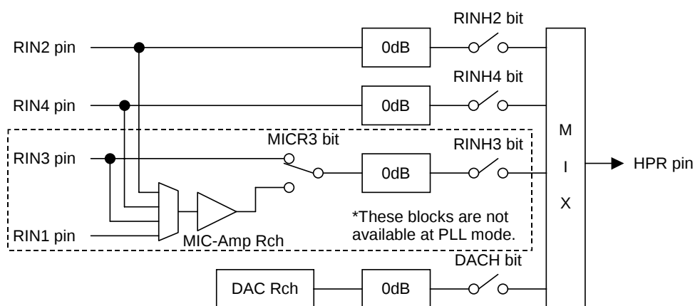
Figure 61. HPR Mixing Circuit (AIN3 bit = "1", HPG bit = "0")
