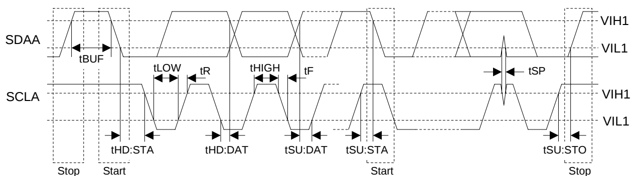
Figure 14. I²C Bus Mode Timing (Audio)
