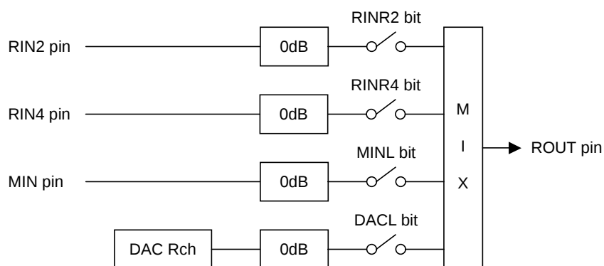
Figure 48. ROUT Mixing Circuit (AIN3 bit = "0", LOVL bit = "0")
