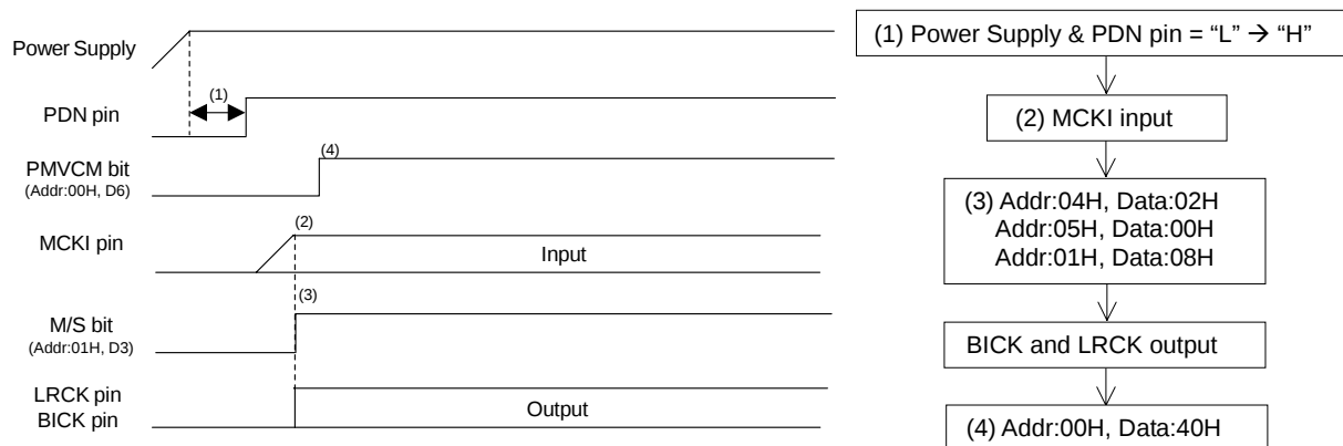
Figure 89. Clock Set Up Sequence (5)
