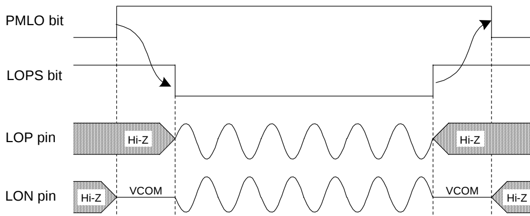
Figure 52. Power-up/Power-down Timing for Mono Line Output
