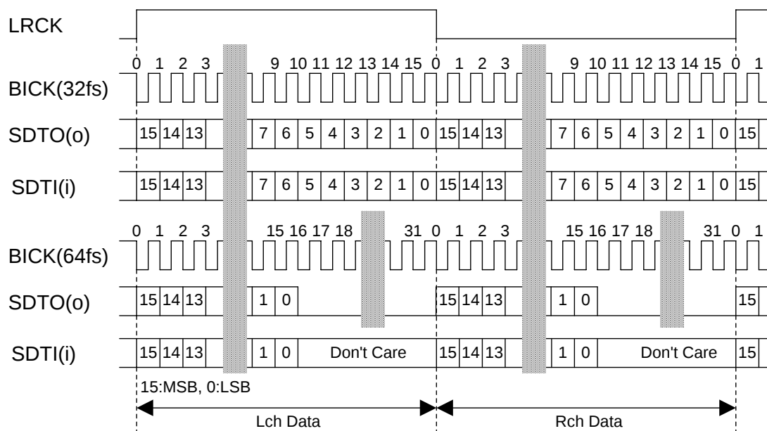
Figure 29. Mode 2 Timing
