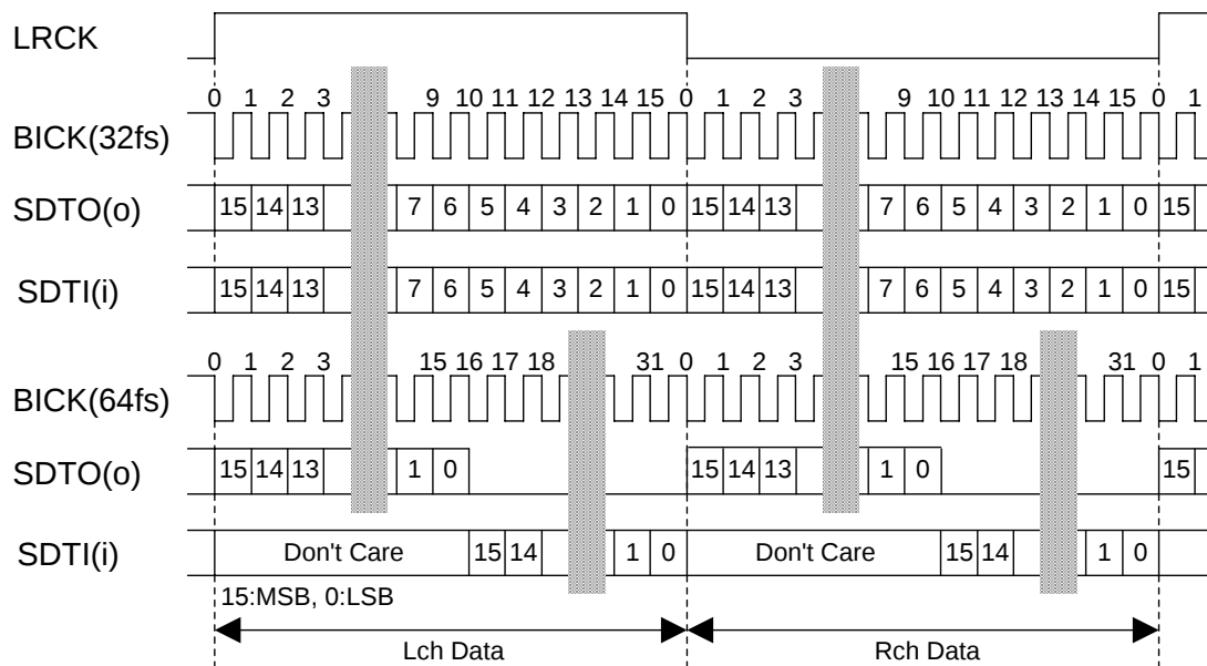
Figure 28. Mode 1 Timing
