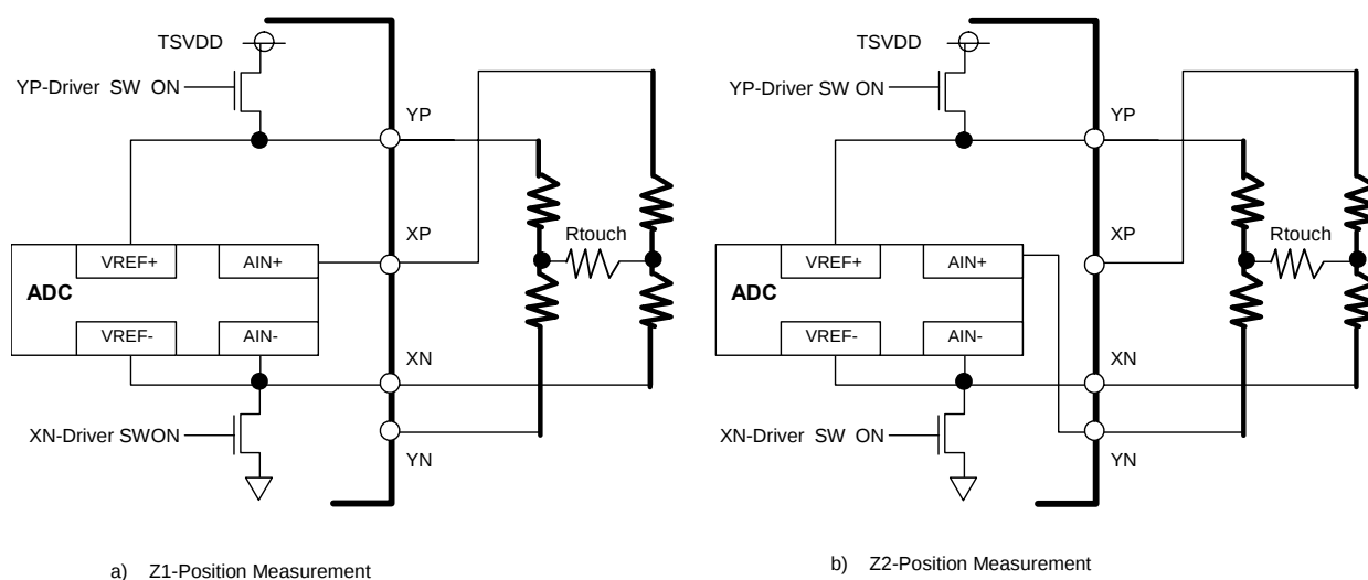
Figure 64 Pen Pressure Measurements
