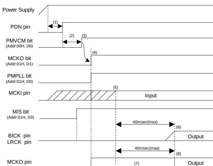
Figure 85. Clock Set Up Sequence (1)
