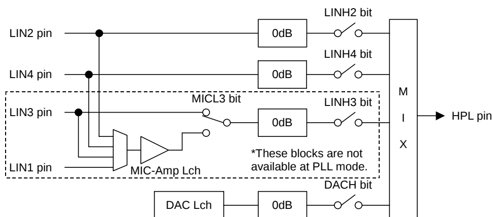
Figure 60. HPL Mixing Circuit (AIN3 bit = "1", HPG bit = "0")
