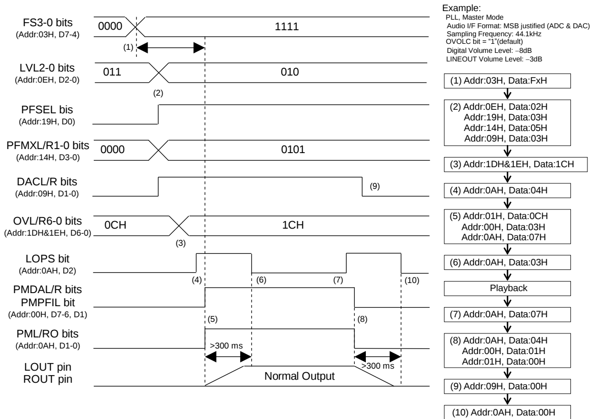
Figure 116. Stereo Lineout Sequence (Lineout Playback: SDTI → Audio I/F → SVOLA → DATT-A → DACL/R → LOUT/ROUT)
