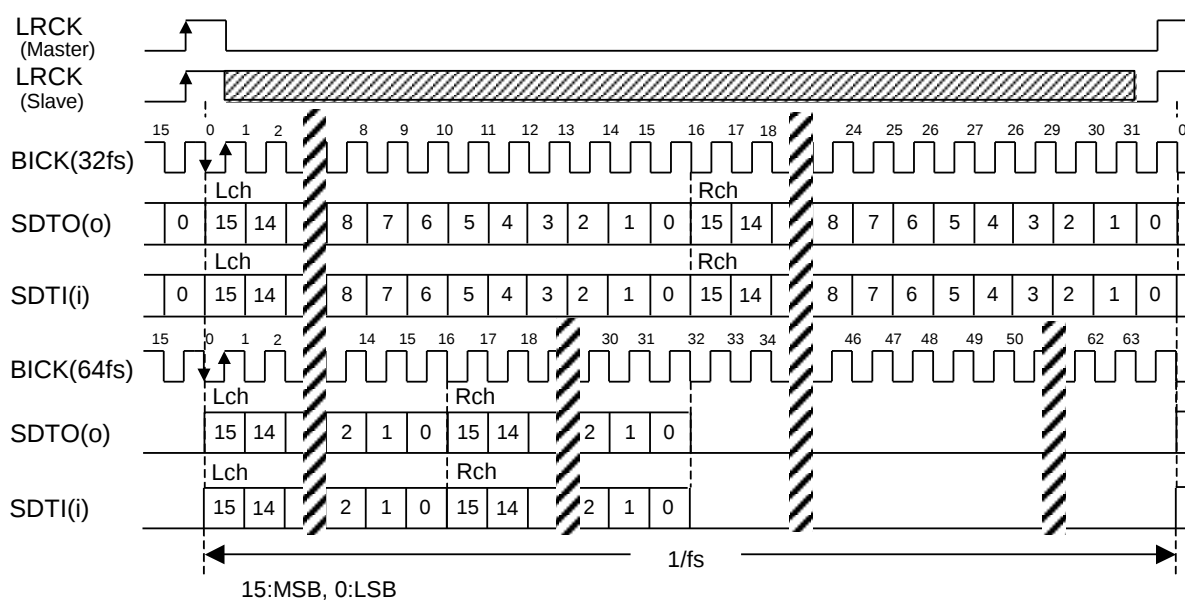
Figure 36. Mode 0 Timing (BCKP bit = "1", MSBS bit = "0")
