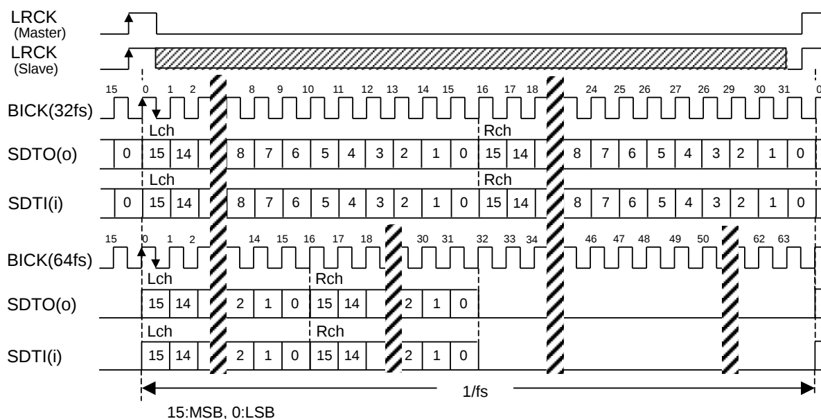
Figure 35. Mode 0 Timing (BCKP bit = "0", MSBS bit = "0")
