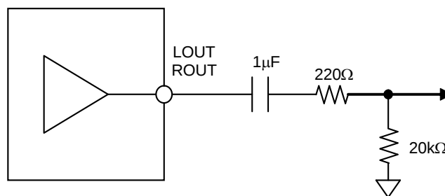
Figure 67. External Circuit for Stereo Line Output (in case of using Pop Noise Reduction Circuit)
