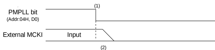
Figure 117. Clock Stopping Sequence (1)
