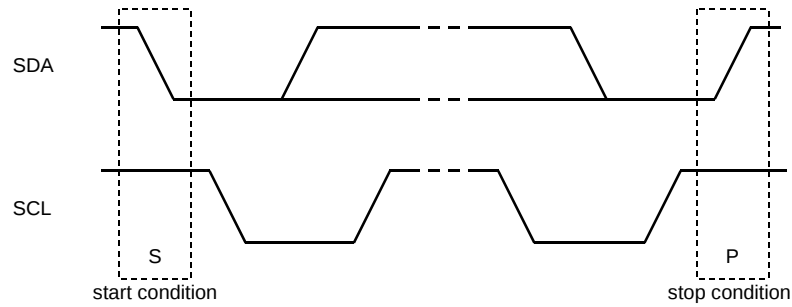
Figure 103. START and STOP Conditions
