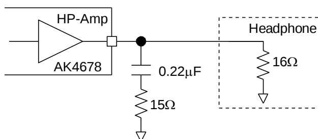
Figure 74. HP-Amp oscillation prevention circuit example
