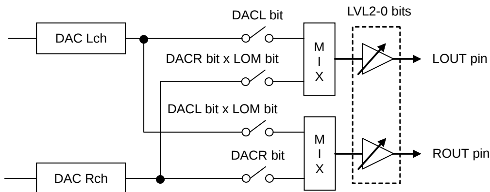
Figure 66. Stereo Line Output
