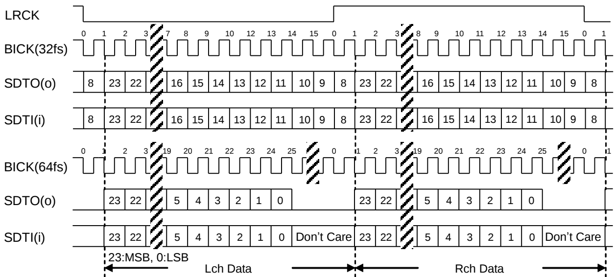
Figure 41. Mode 3 Timing
