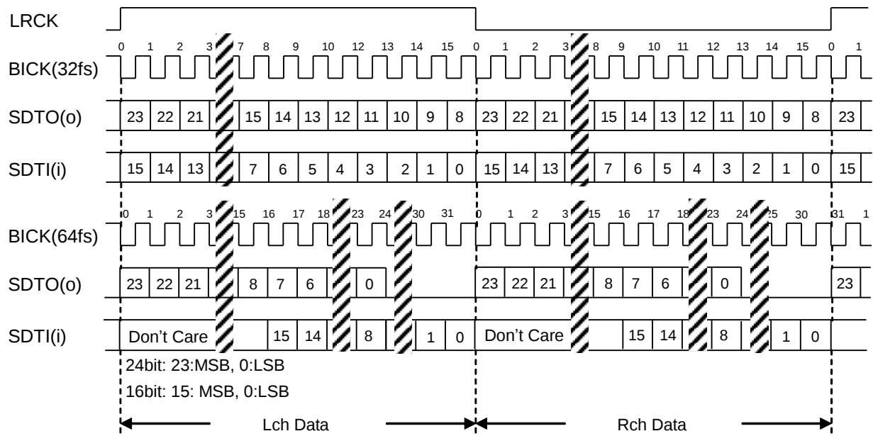
Figure 39. Mode 1 Timing
