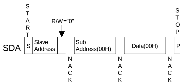
Figure 34. Dummy Command
