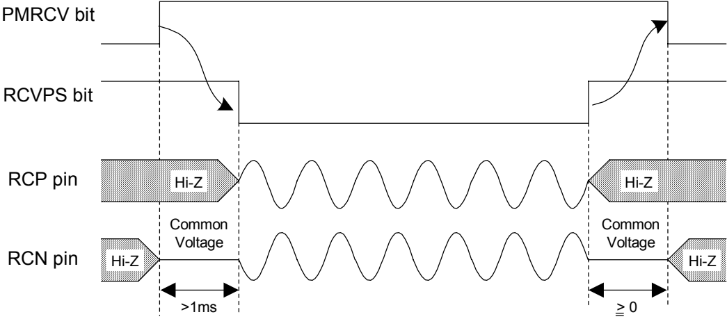
Figure 83. Power-up/Power-down Timing for Receiver-Amp
