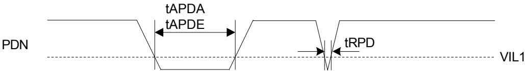
Figure 35. Power Down & Reset Timing 2
