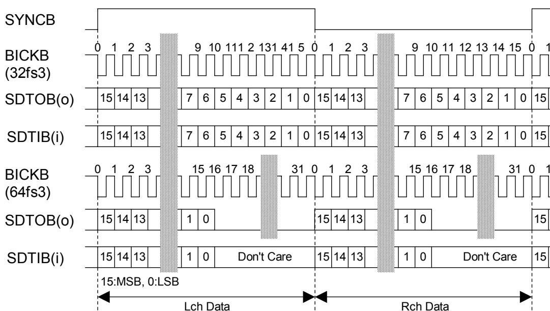
Figure 105. Timing of MSB justified (PCM I/F B)
