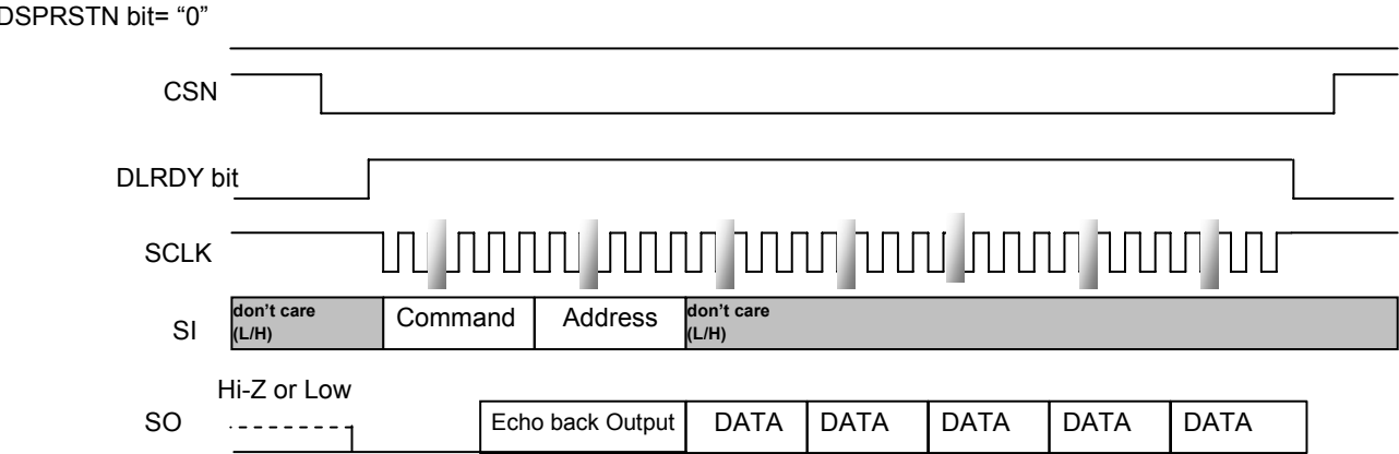
Figure 145. RAM Reading at Consecutive Address
