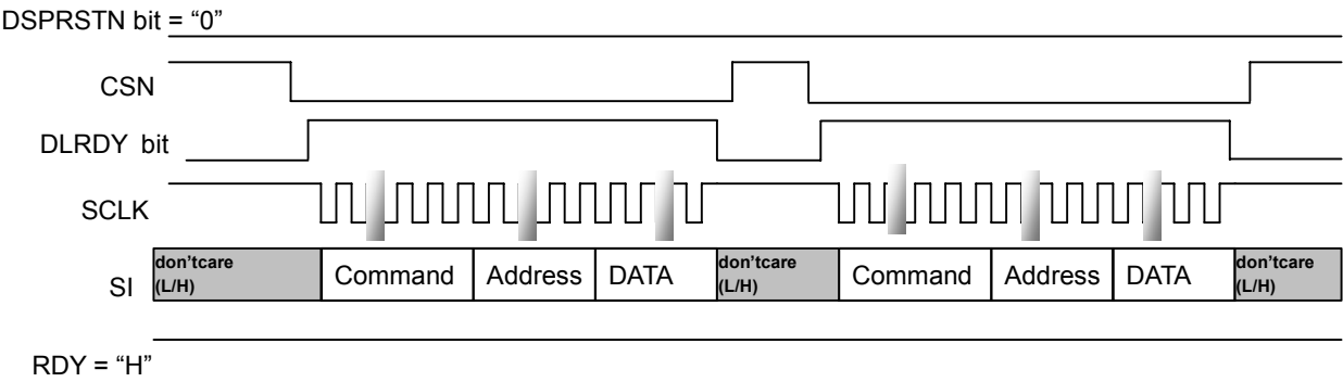
Figure 139. Writing to RAM at specified Address Locations
