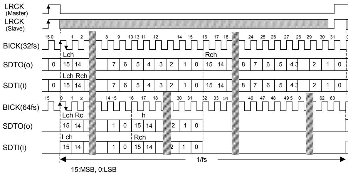
Figure 48. Mode 0 Timing (BCKP bit = "0", MSBS bit = "1")
