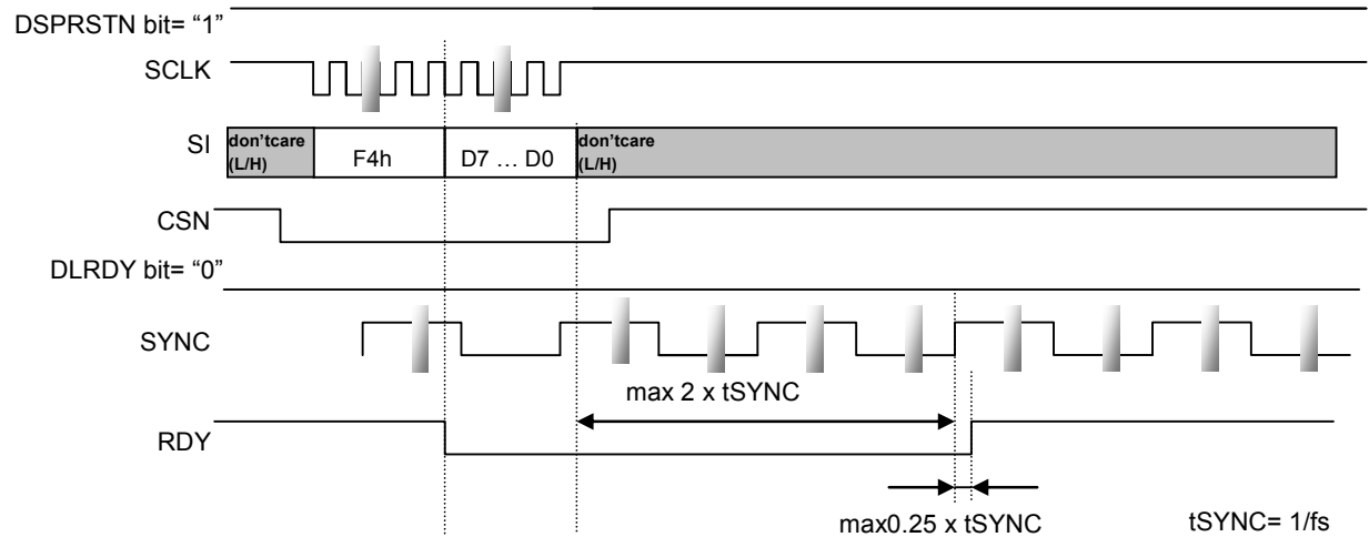
Figure 144. External Conditional Jump Timing (during RUN)
