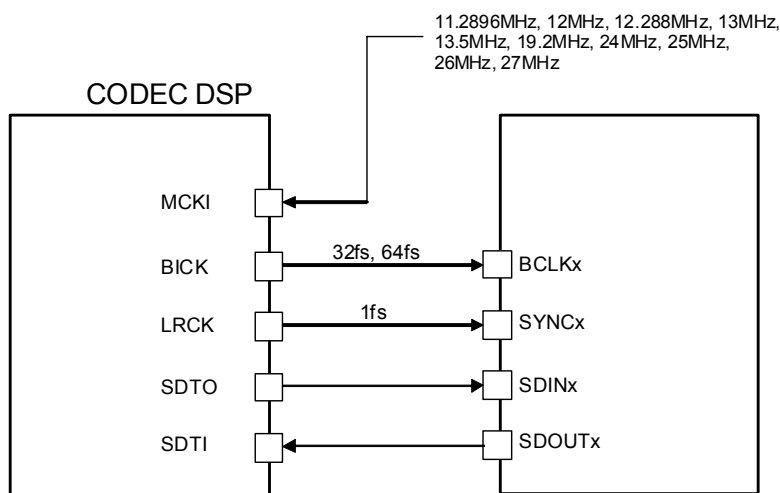
Figure 39. PLL Master Mode (x=1 to 4)
