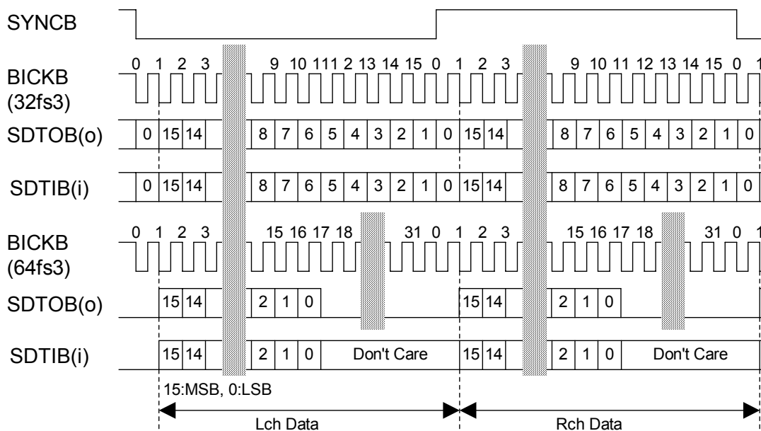
Figure 107. Timing of I 2 S (PCM I/F B)
