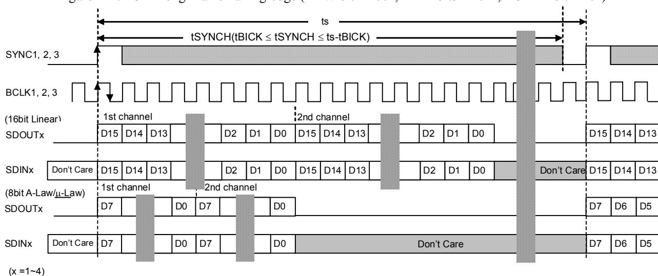
Figure 112. PCM Long Frame Falling-edge (LAW bit = "00", DIFD bits = "01", BCKPD bit = "0")
