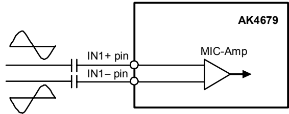
Figure 55. Connection Example for Full-differential Mic Input (MDIF1/2/3 bits = "1")
