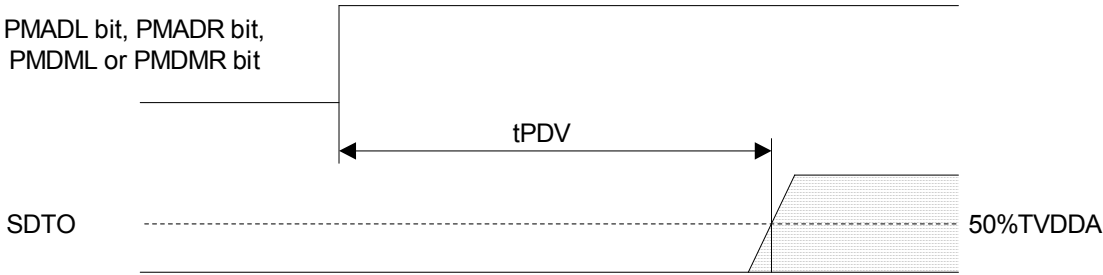
Figure 34. Power Down & Reset Timing 1
