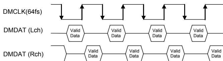
Figure 60. Data In/Output Timing with Digital MIC (DCLKP bit = “0”)
