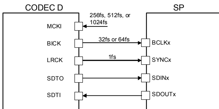
Figure 42. EXT Master Mode (x=1 to 4)
