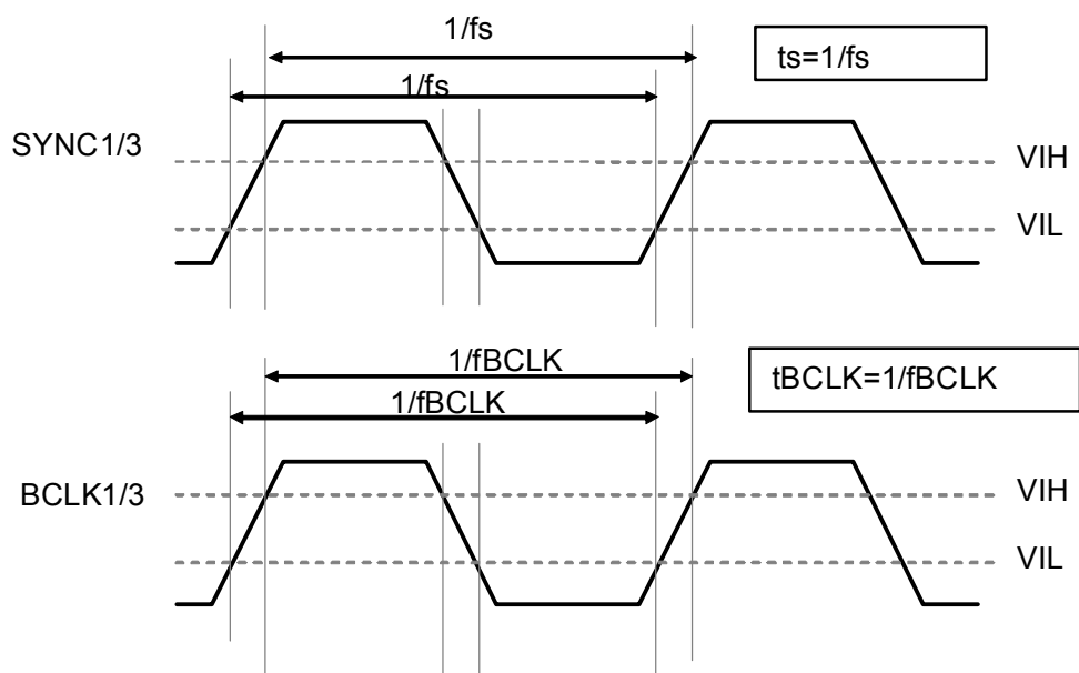
Figure 27. System Clock
