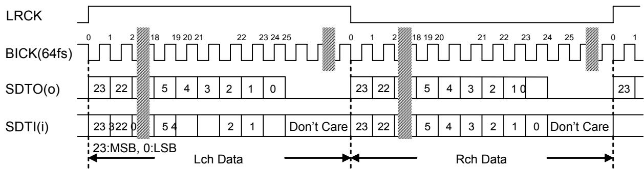
Figure 51. Mode 2 Timing
