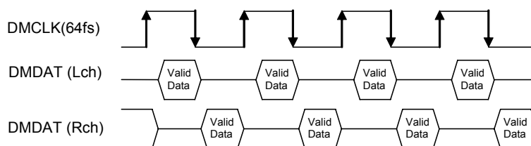
Figure 59. Data In/Output Timing with Digital MIC (DCLKP bit = “1”)
