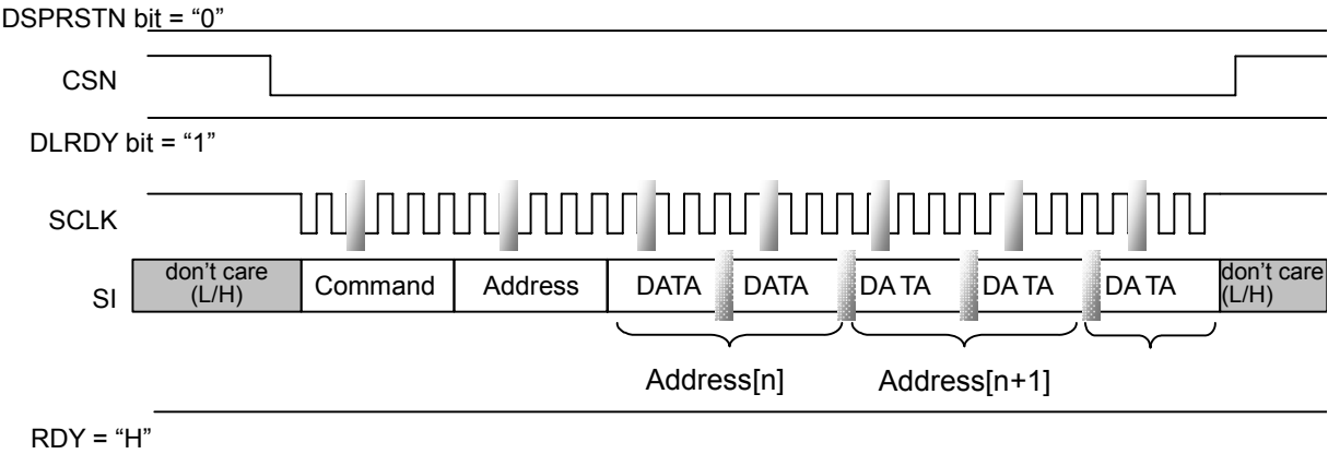
Figure 138. Writing to RAM at Consecutive Address Locations
