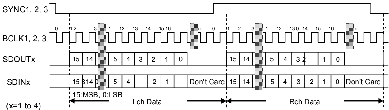
Figure 116. I 2 S Format (LAW bits = "00", DIFD bits = "11")
