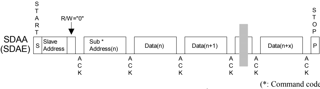
Figure 123. Data Transfer Sequence at the I 2 C-Bus Mode
