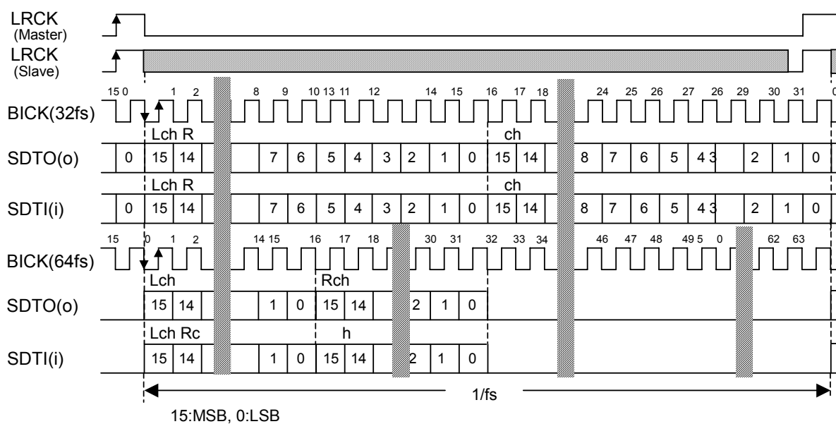
Figure 49. Mode 0 Timing (BCKP bit = "1", MSBS bit = "1")
