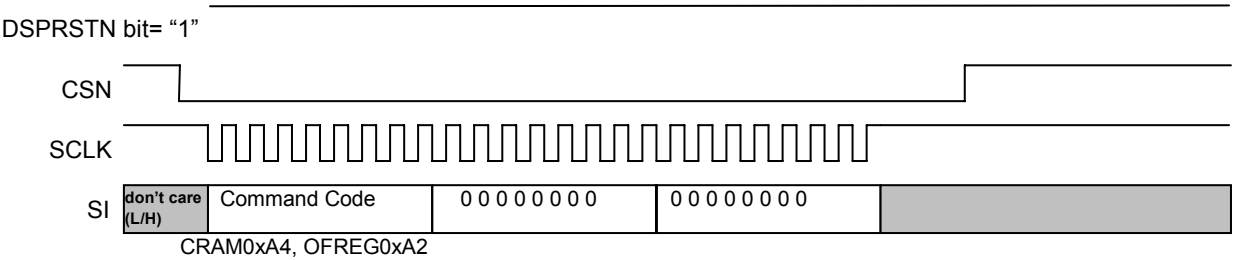
Figure 142. CRAM/OFREG Write
