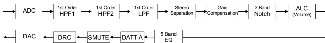
Figure 63. Path at Recording Mode 1 &amp; Playback Mode 2
