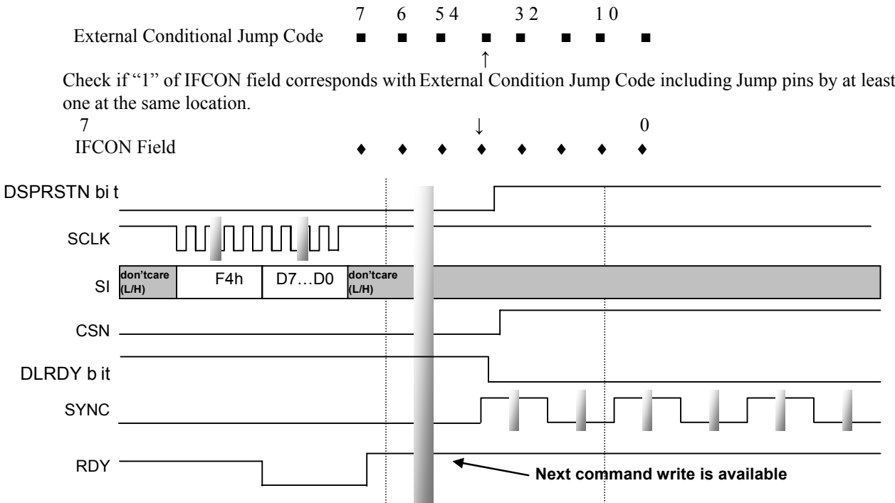
Figure 143. External Conditional Timing (in DSP Reset)
