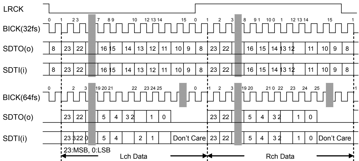
Figure 52. Mode 3 Timing
