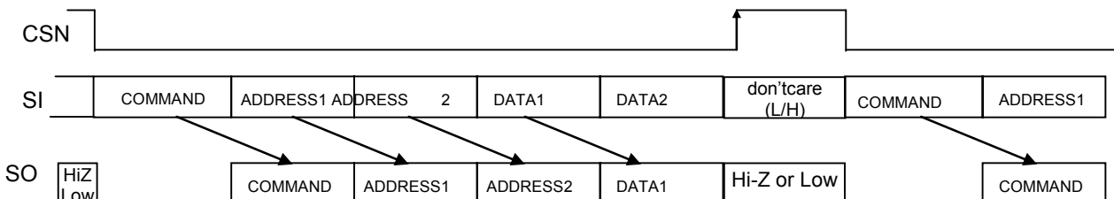
Figure 135. Echo-Back Writing 1
