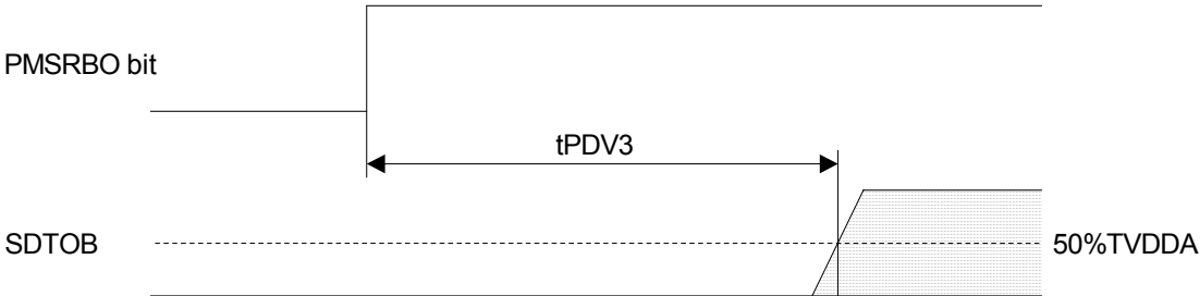
Figure 37. Power Down & Reset Timing 4
