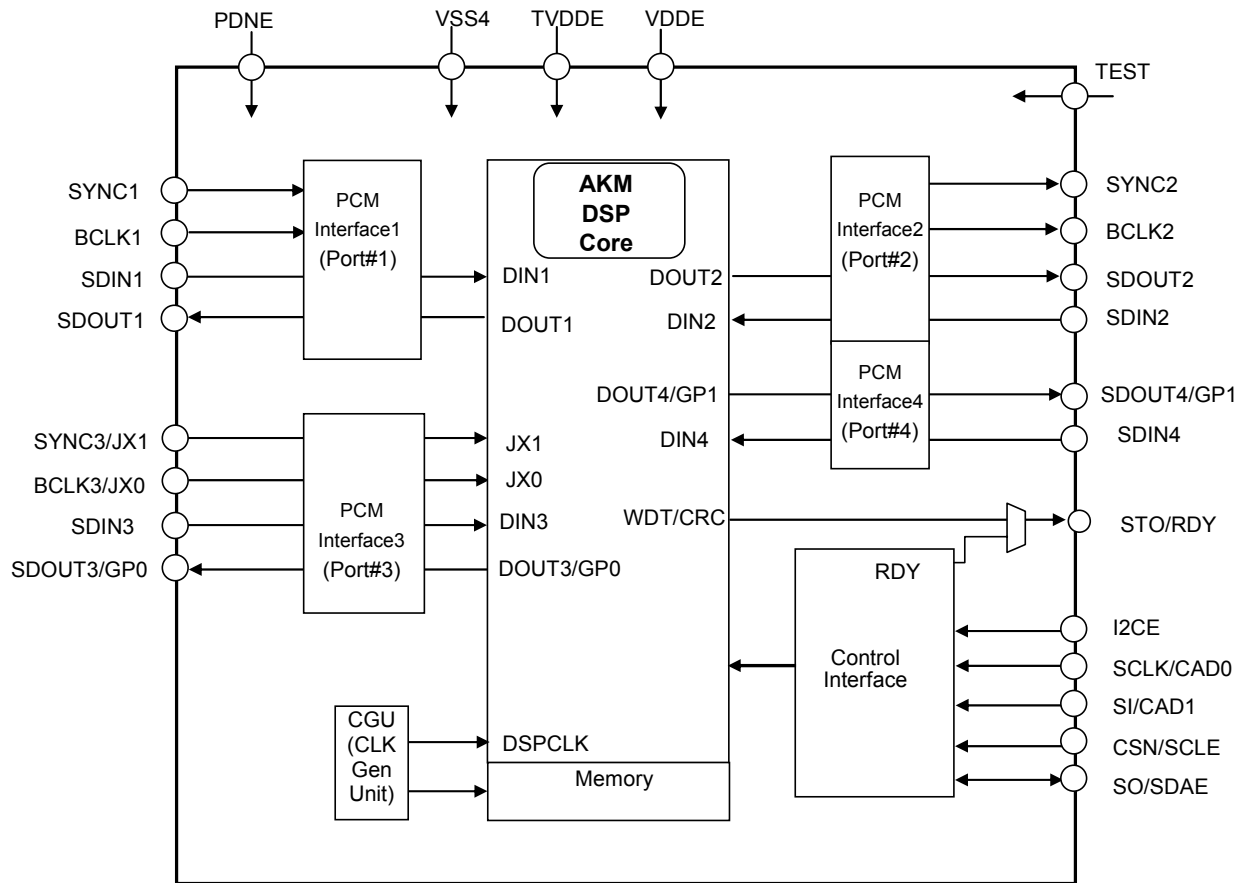
Figure 3. DSP Block Diagram
