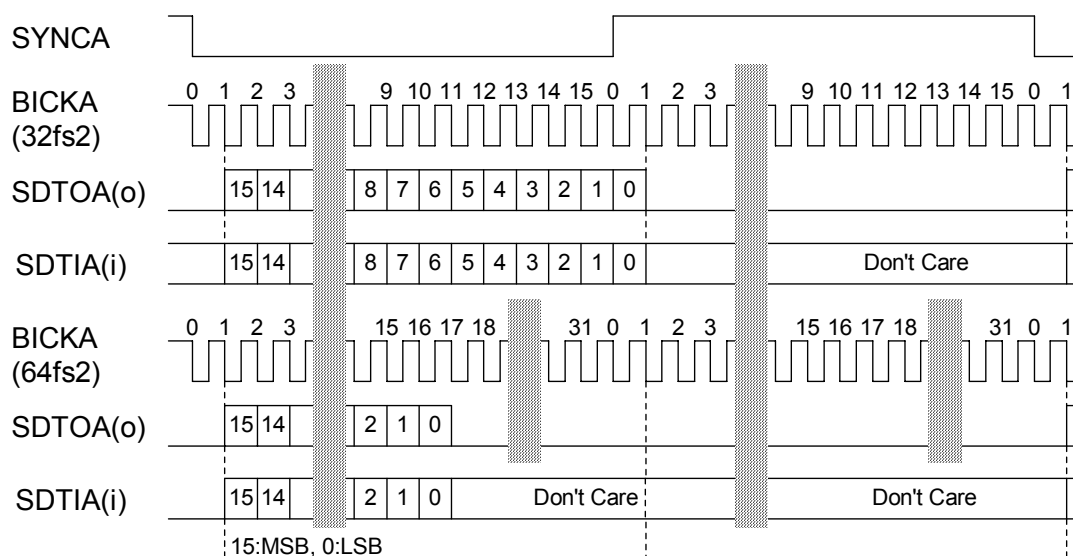
Figure 106. Timing of I 2 S (PCM I/F A)
