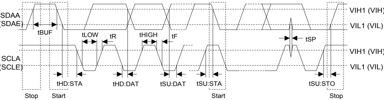
Figure 30. I²C Bus Mode Timing
