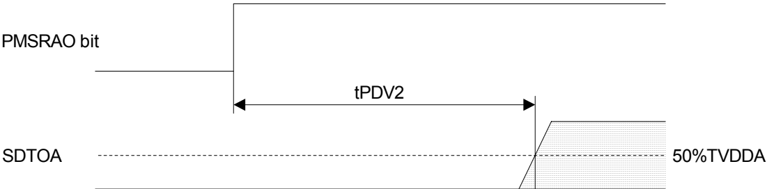
Figure 36. Power Down & Reset Timing 3
