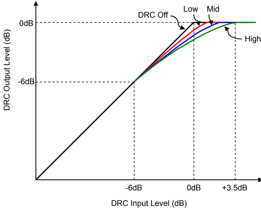
Figure 75. DRC Gain Curve
