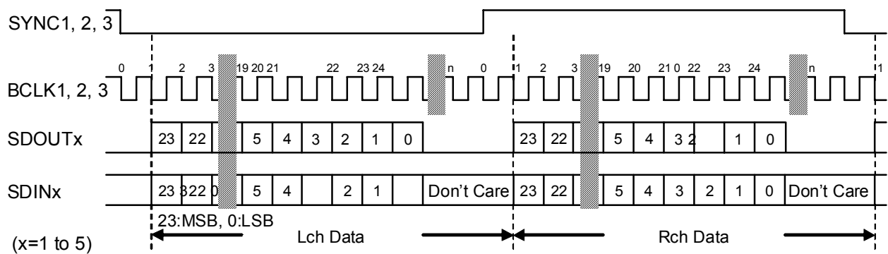
Figure 117. I 2 S Format (LAW bits = "01", DIFD bits = "11")
