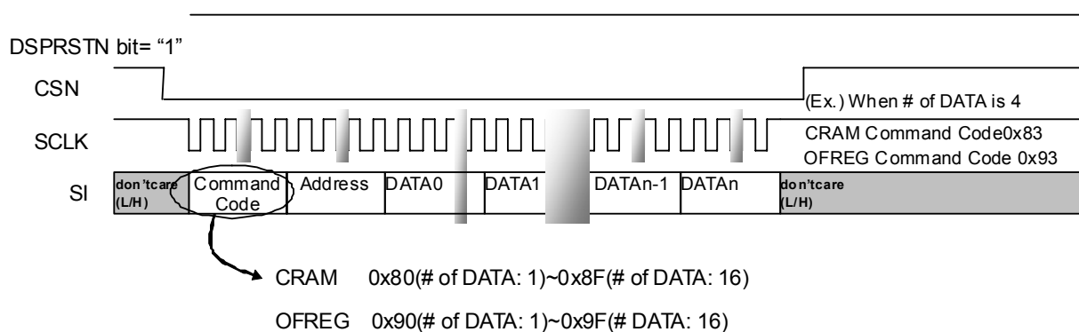
Figure 140. CRAM/OFREG Write Preparation
