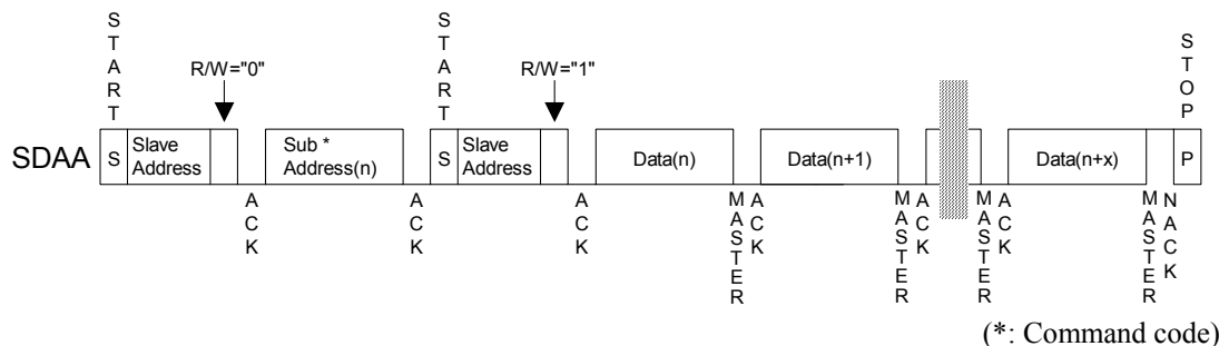
Figure 129. RANDOM ADDRESS READ (Audio Block)
