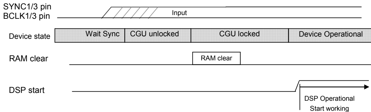
Figure 122. RAM Clear Sequence
