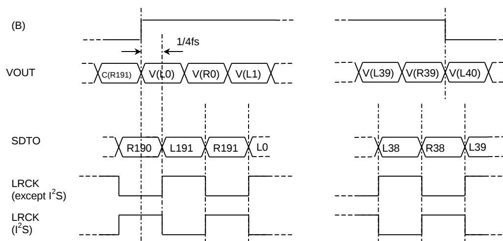
Figure 27. V output timings
