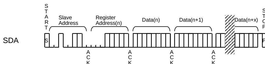
Figure 47. WRITE Operation
