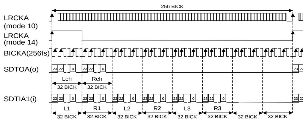
Figure 14. Mode 10 ,14 Timing
