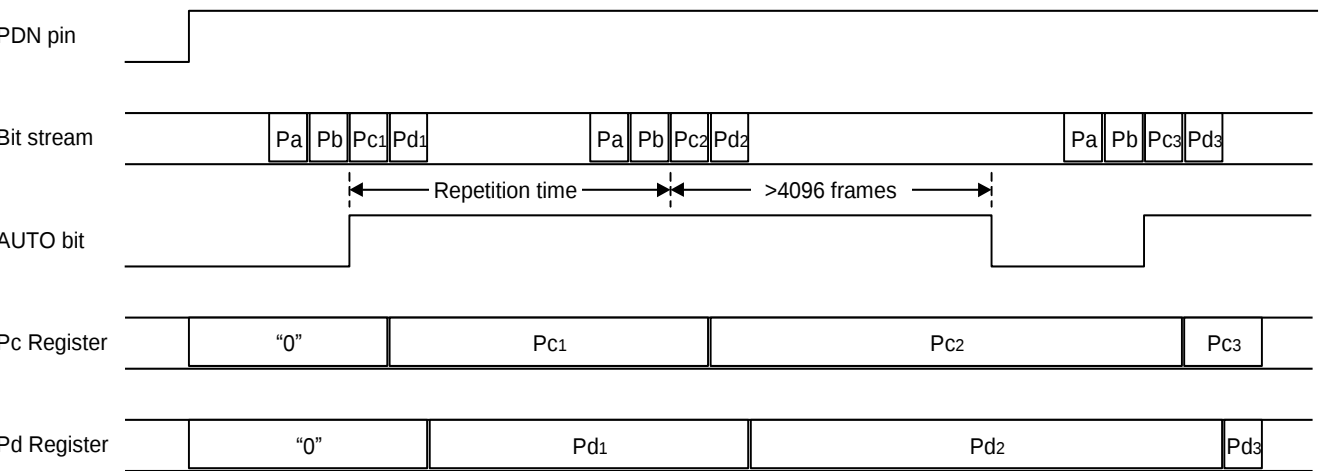
Figure 38. Timing example 1
