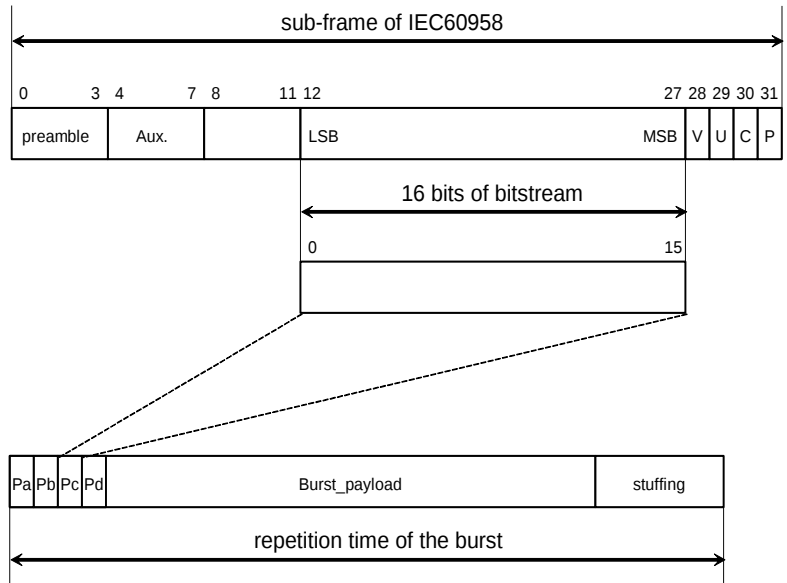
Figure 37. Data structure in IEC60958
