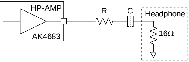
Figure 26. External Circuit Example of Headphone
