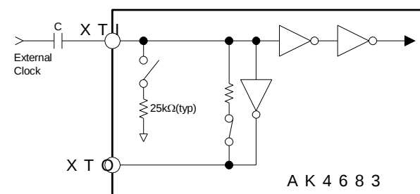
Figure 5. AC-coupled Input
