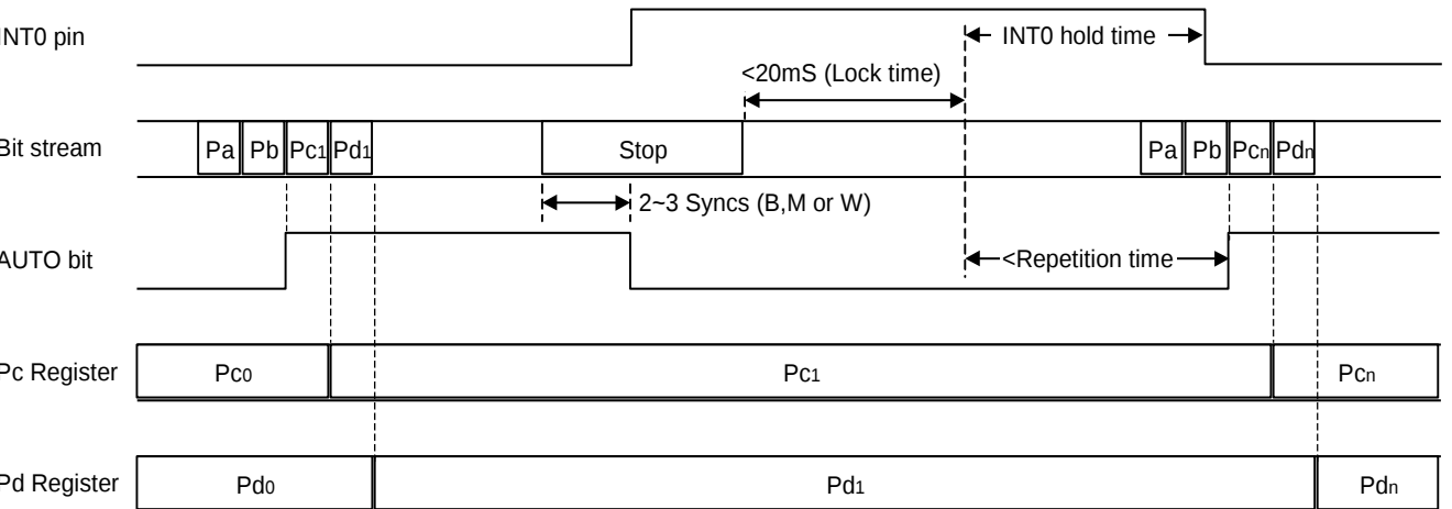
Figure 39. Timing example 2
