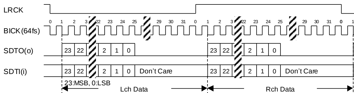
Figure 11. Mode 3 ,7 Timing
