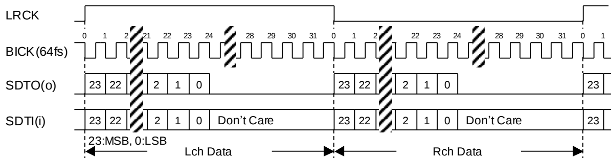
Figure 10. Mode 2,6 Timing
