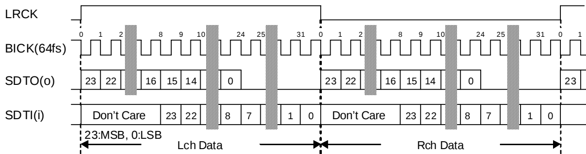
Figure 6. Audio Data Timing (SDTO: Mode0/2, SDTI: Mode1)
