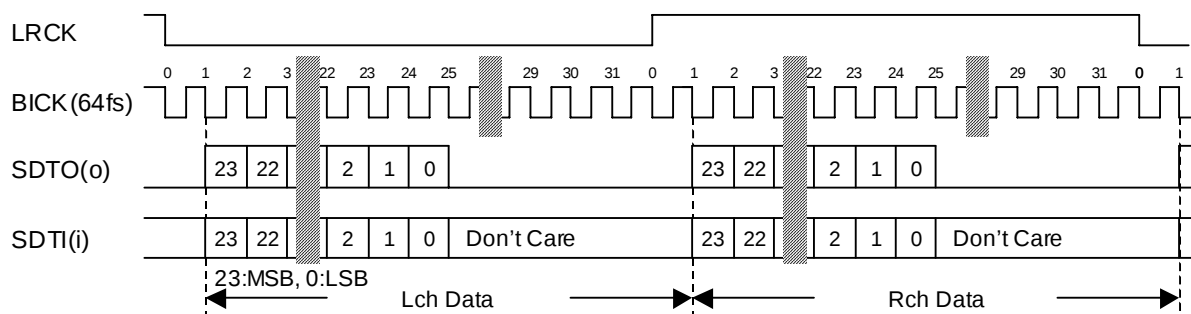
Figure 8. Audio Data Timing (SDTO: Mode1/3, SDTI: Mode3)
