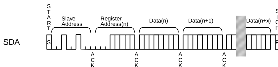
Figure 25. WRITE Operation
