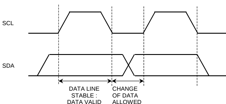
Figure 19. Data Transfer
