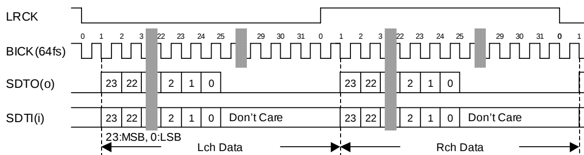
Figure 5. Mode 3/7 Timing
