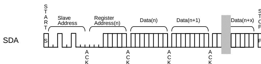
Figure 15. WRITE Operation
