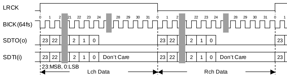
Figure 4. Mode 2/6 Timing
