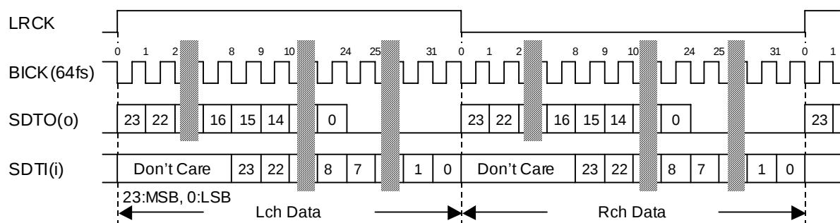
Figure 3. Mode 1/5 Timing
