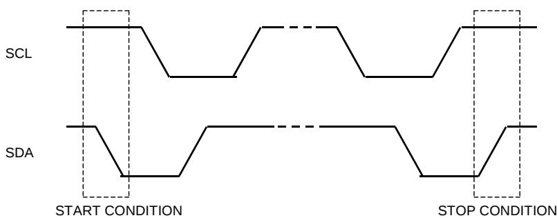
Figure 10. START and STOP conditions
