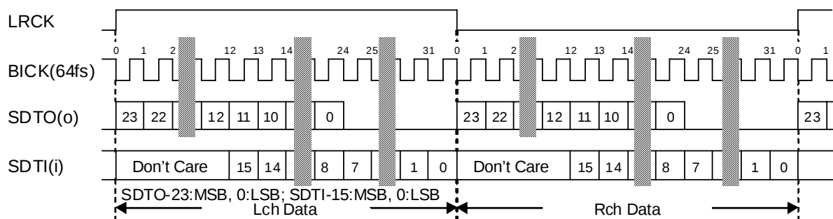
Figure 2. Mode 0/4 Timing
