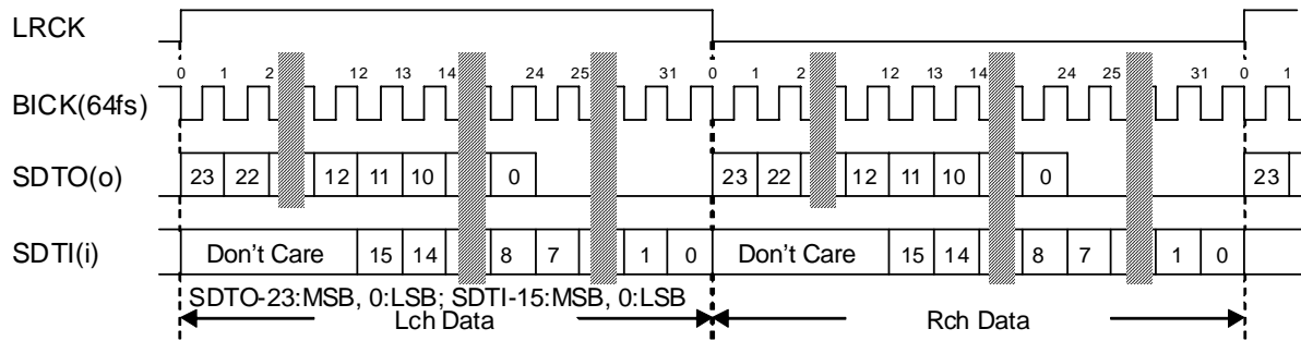
Figure 3. PORT1= Mode0/2, PORT2=Mode0 Timing
