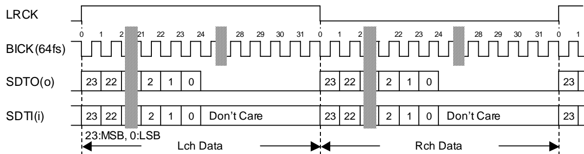
Figure 5. PORT1= Mode0/2, PORT2=Mode2 Timing
