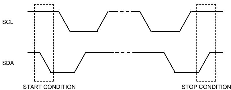
Figure 13. START and STOP Conditions
