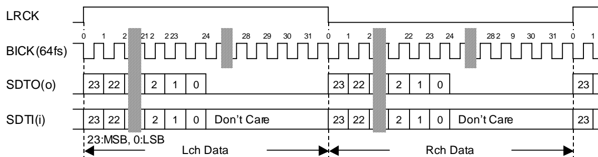
Figure 6. PORT1= Mode0/2, PORT2=Mode2 Timing
