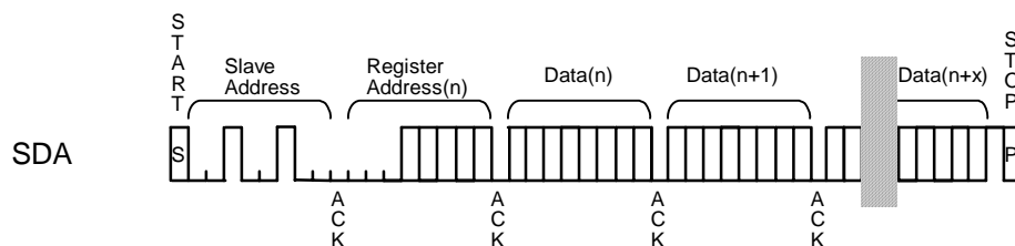
Figure 18. WRITE Operation
