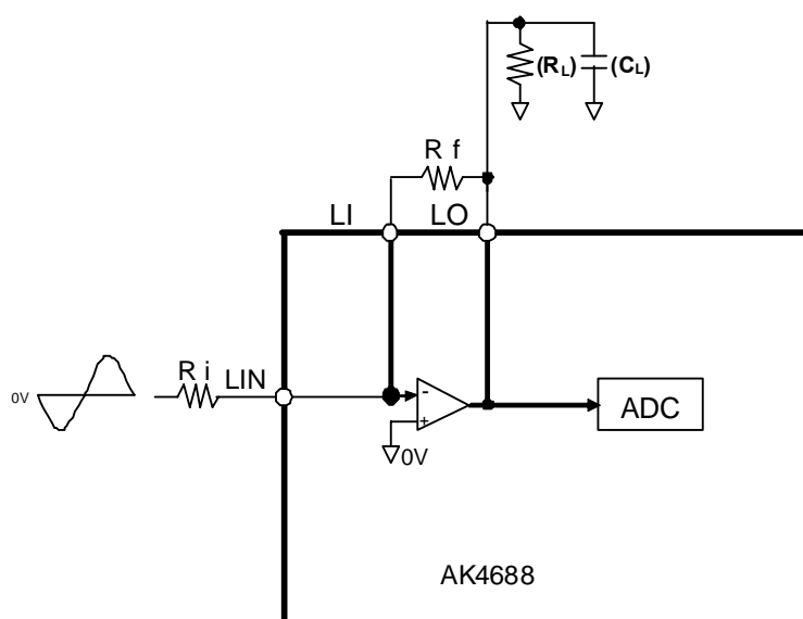
Figure 3. External Circuit of Pre-Amp
