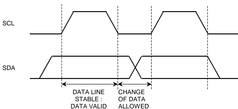
Figure 12. Data Transfer
