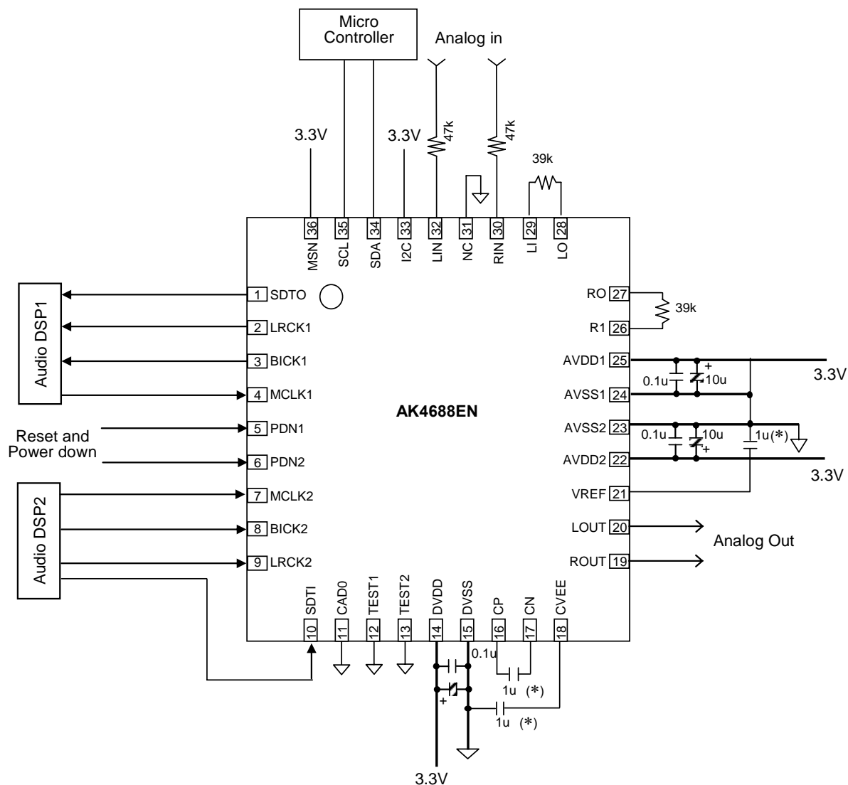
Figure 21. Typical Connection Diagram (I²C Control mode, CAD0 pin = "L", Master mode)
