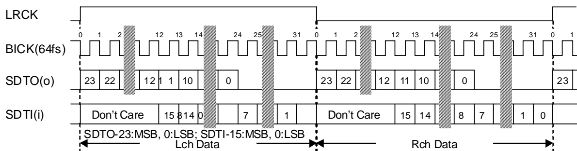
Figure 4. PORT1= Mode0/2, PORT2=Mode0 Timing
