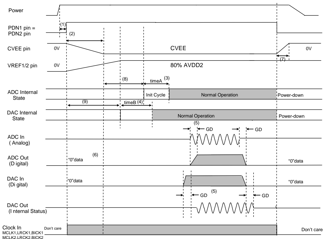
Figure 11. Power-up/down sequence example
