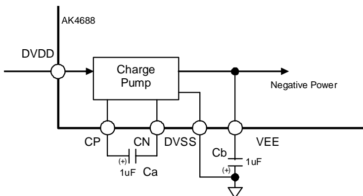
Figure 9. Charge Pump Circuit
