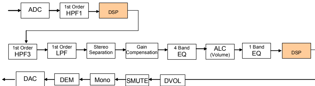
Figure 40. The Path in Loopback Mode 1
