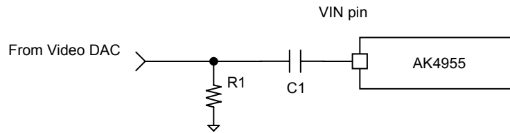
Figure 2. External Resistor of Video Signal Input pin
